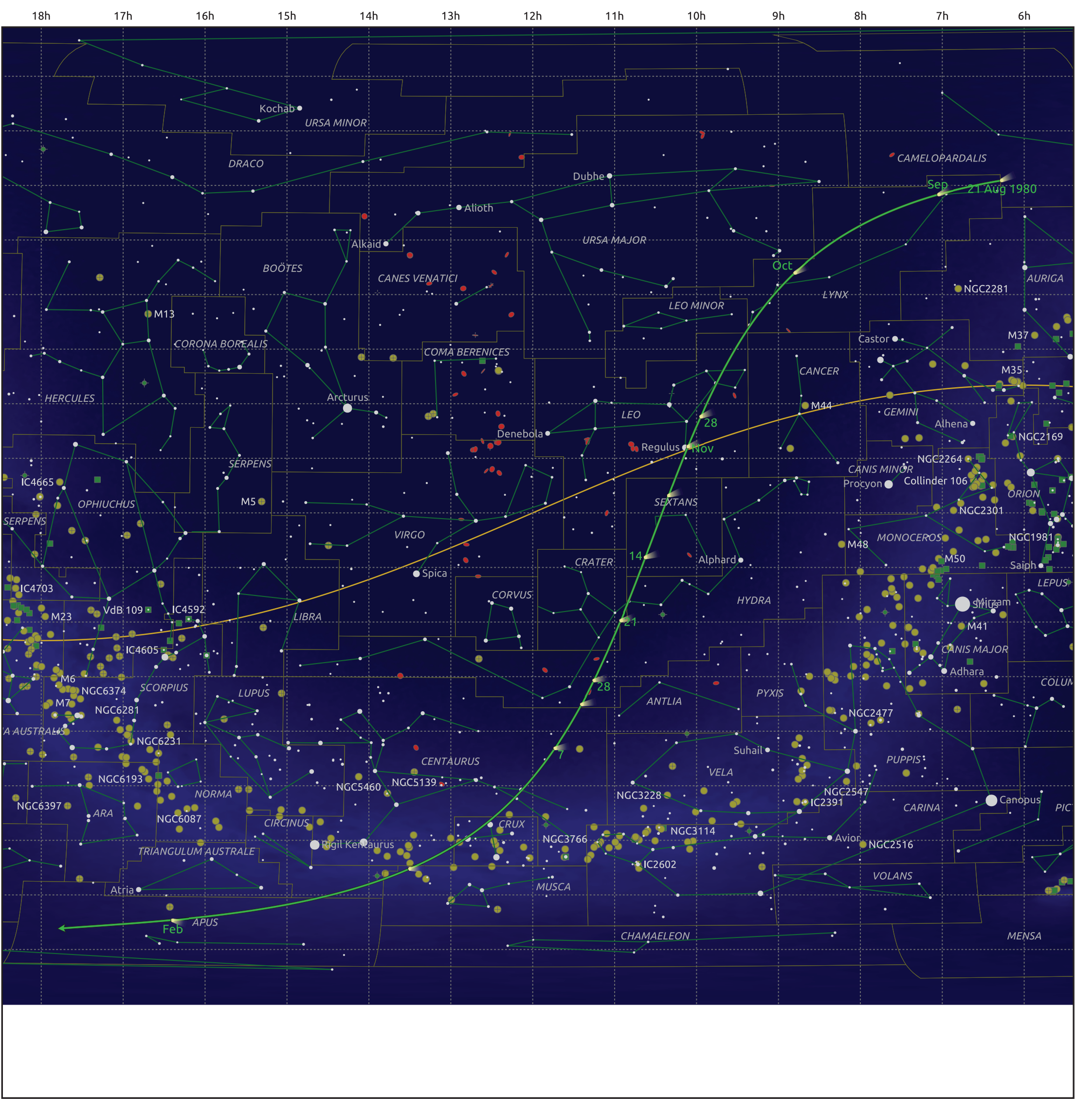
The path of 8P/Tuttle starting on 21 Aug 1980
