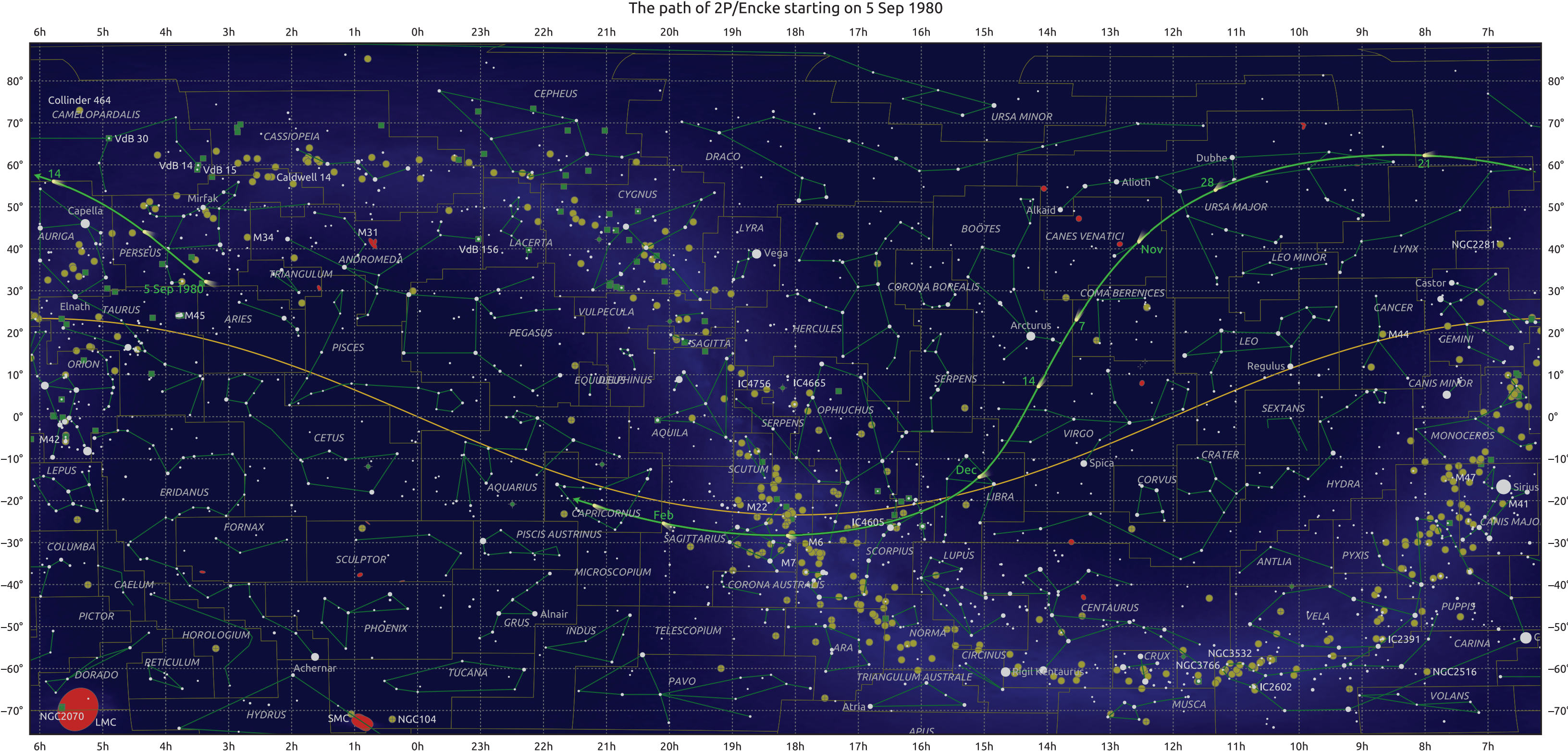
The path of 2P/Encke starting on 5 Sep 1980
