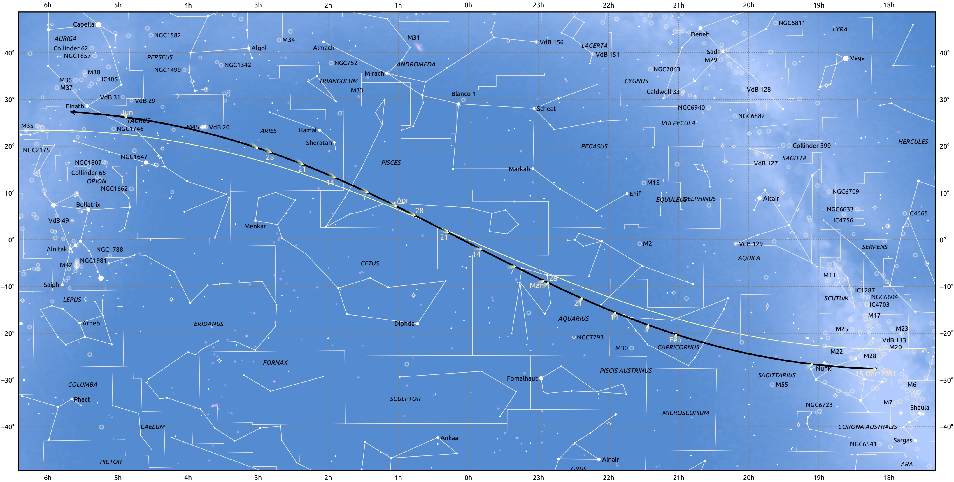
The path of 15P/Finlay starting on 15 Dec 1981
