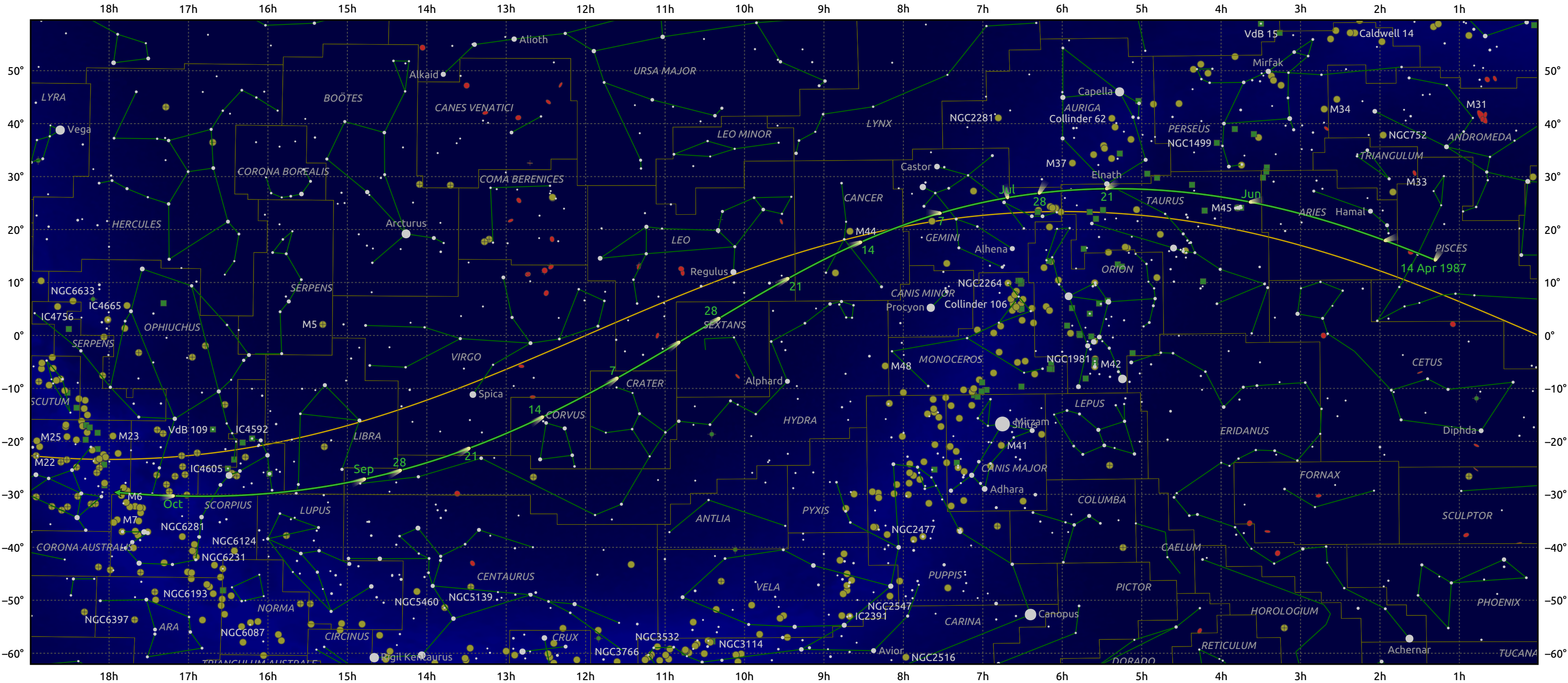
The path of 2P/Encke starting on 14 Apr 1987
