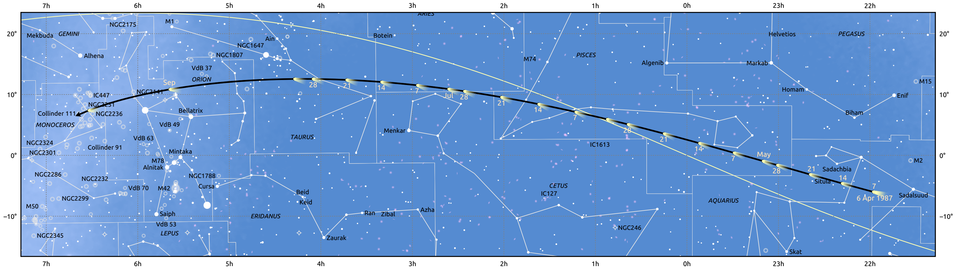
The path of 58P/Jackson-Neujmin starting on 6 Apr 1987
