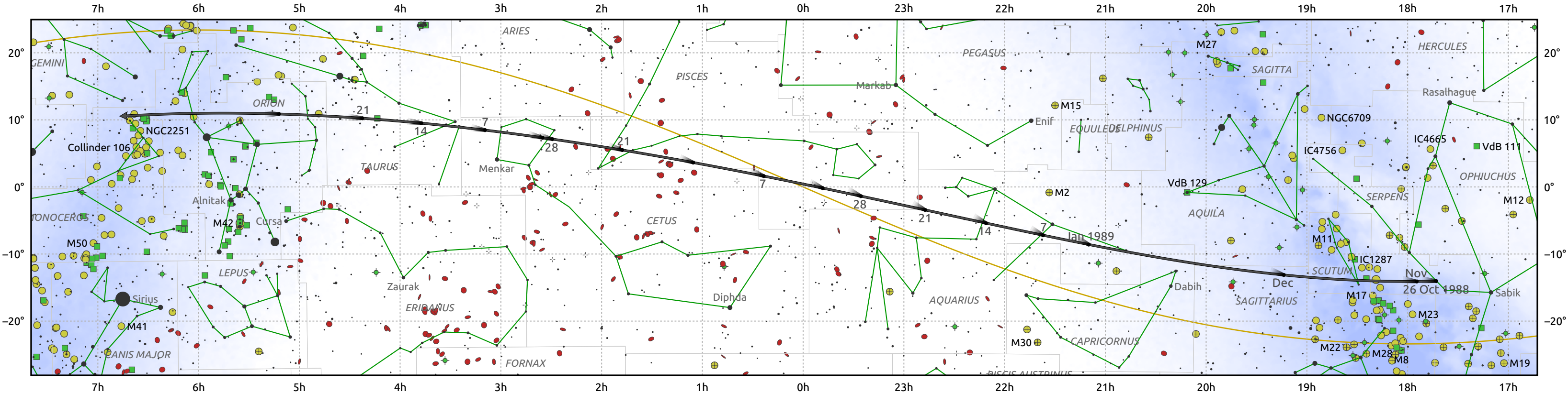
The path of 141P/Machholz starting on 26 Oct 1988
