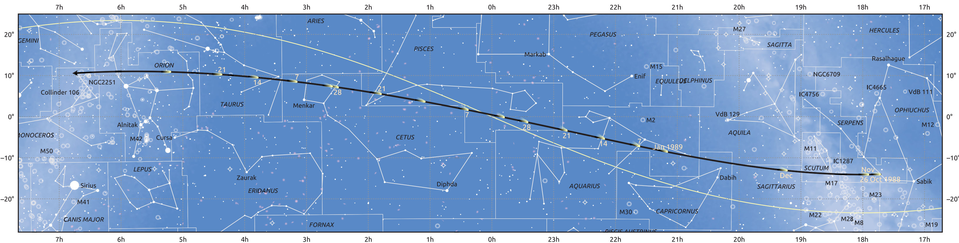
The path of 141P/Machholz starting on 26 Oct 1988
