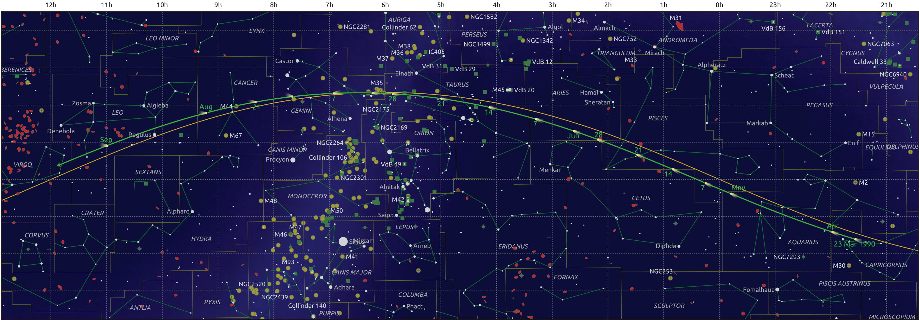
The path of 45P/Honda-Mrkos-Pajdusakova starting on 23 Mar 1990
