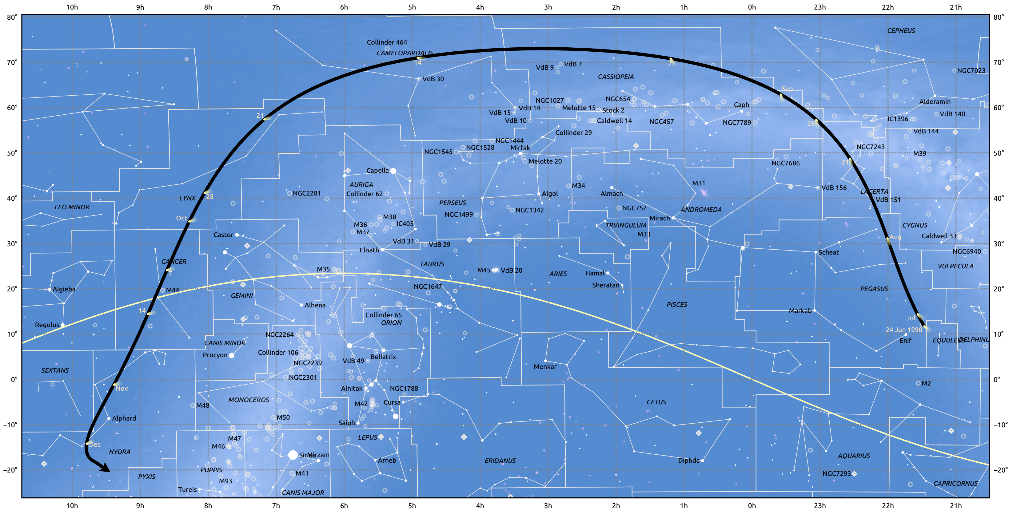
The path of 185P/Petrew starting on 24 Jun 1990
