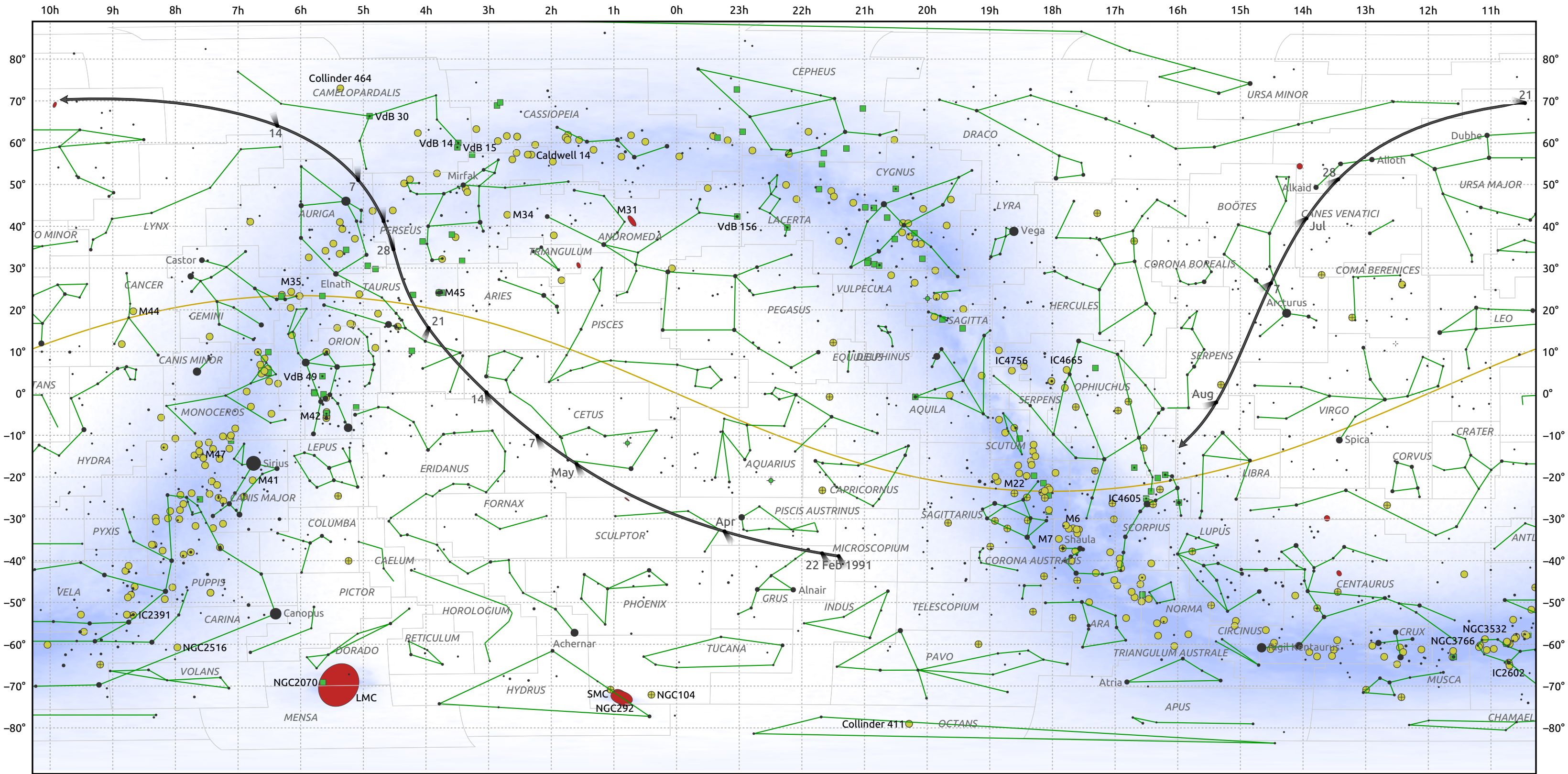
The path of 96P/Machholz starting on 22 Feb 1991
