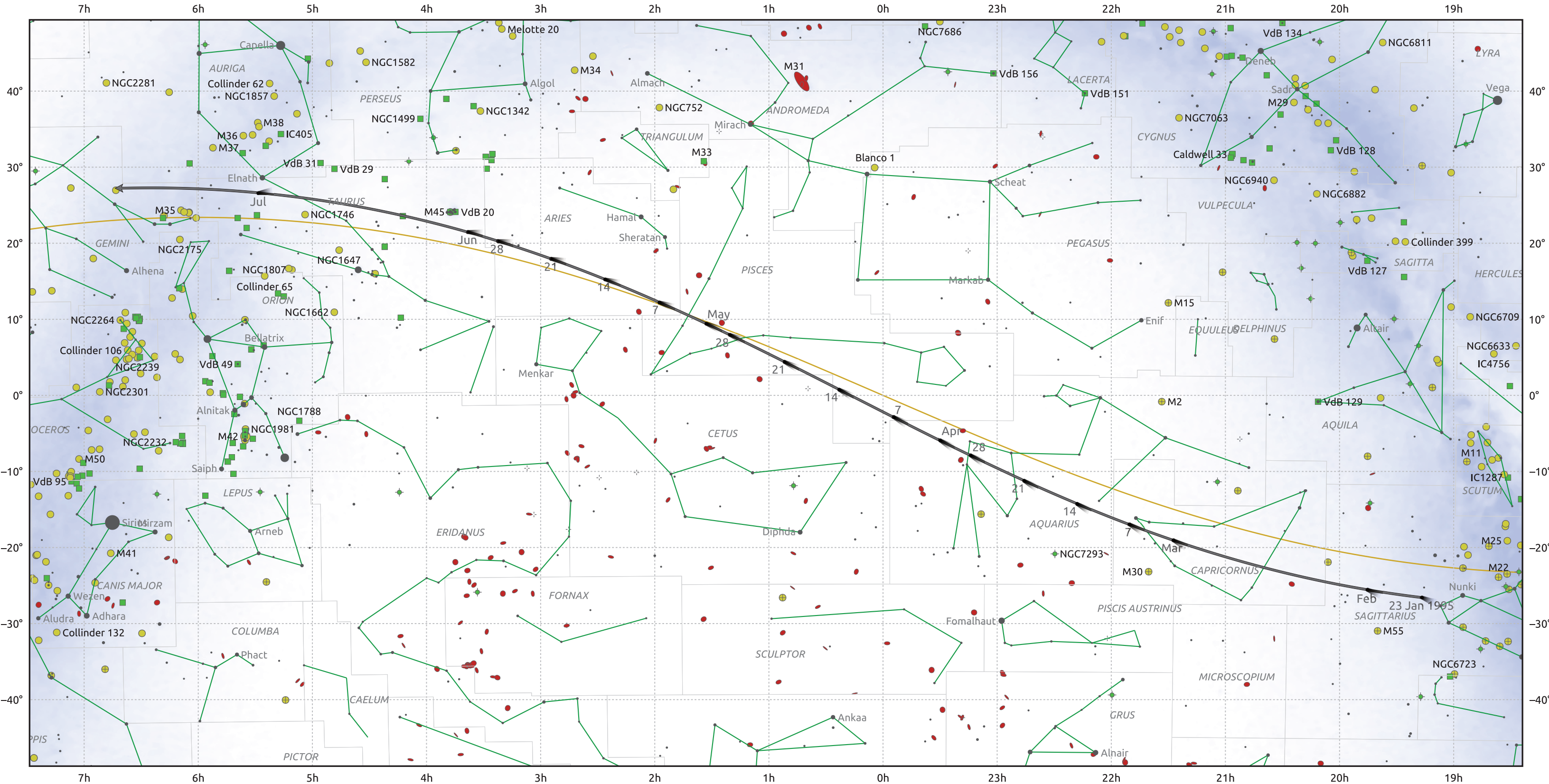
The path of 15P/Finlay starting on 23 Jan 1995
