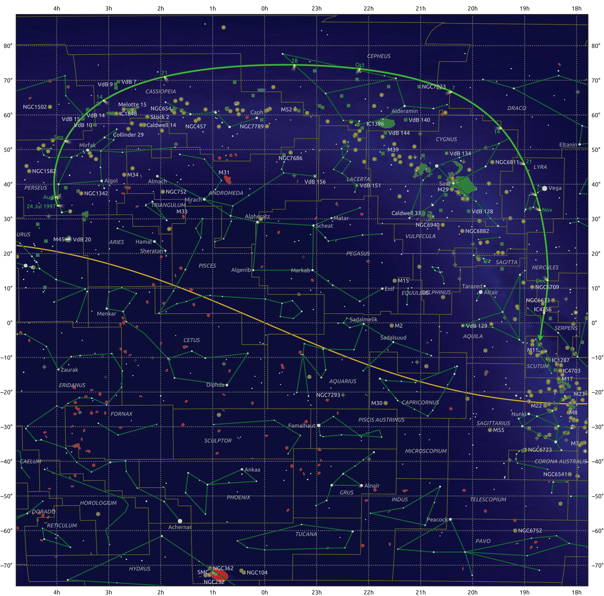
The path of C/1997 T1 (Utsunomiya) starting on 24 Jul 1997
