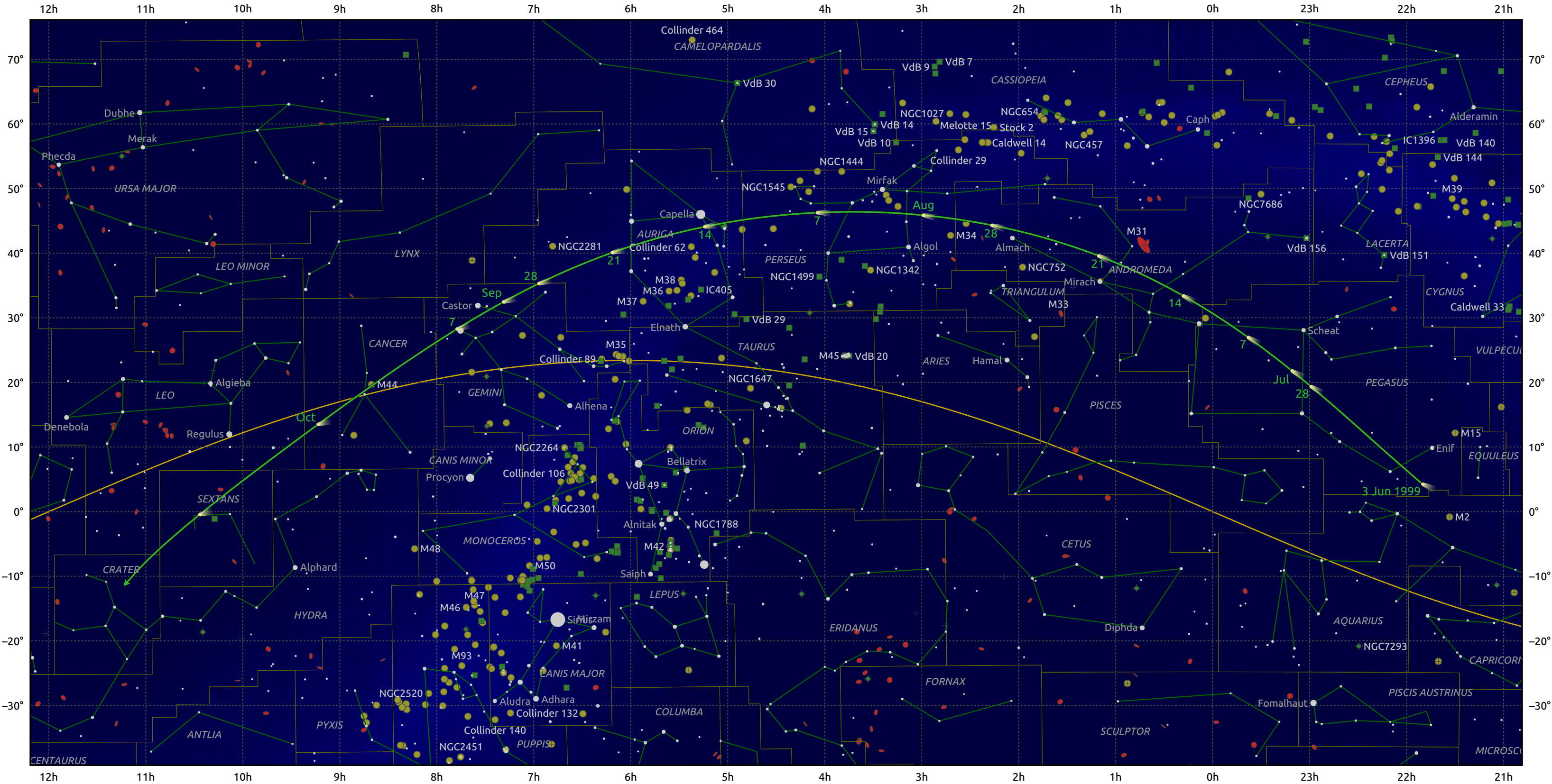
The path of 141P/Machholz starting on 3 Jun 1999
