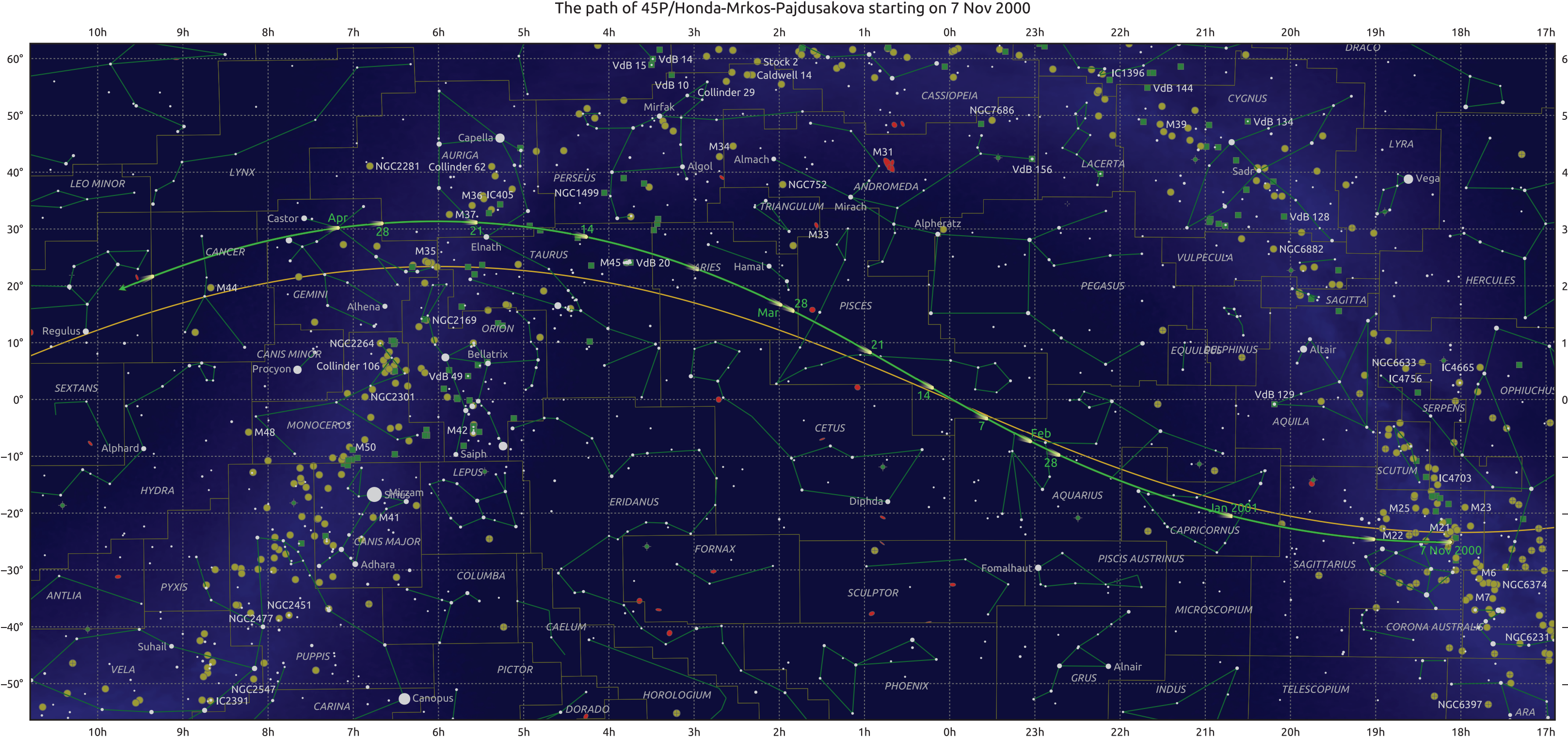
The path of 45P/Honda-Mrkos-Pajdusakova starting on 7 Nov 2000
