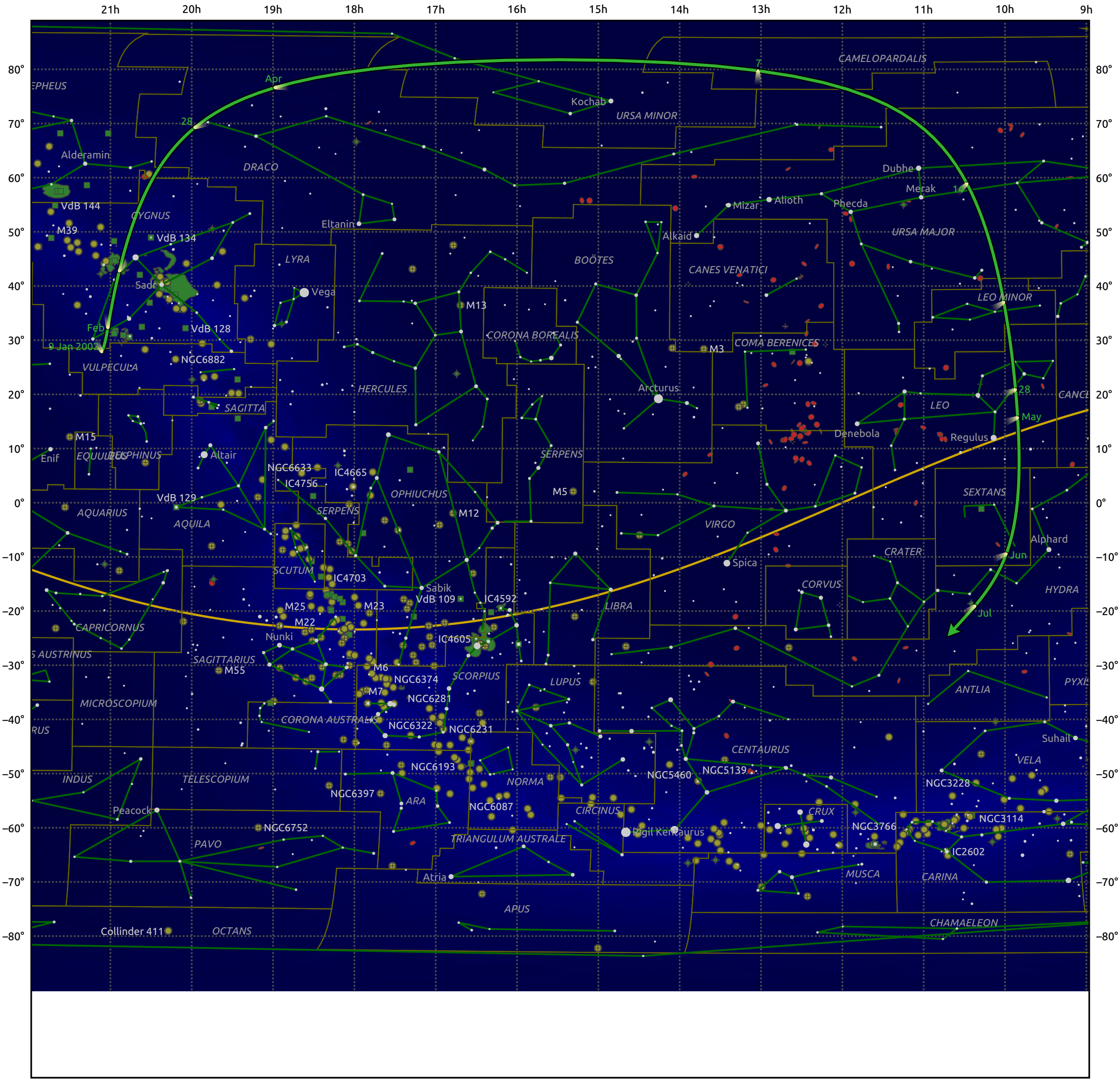
The path of C/2001 OG108 (LONEOS) starting on 9 Jan 2002
