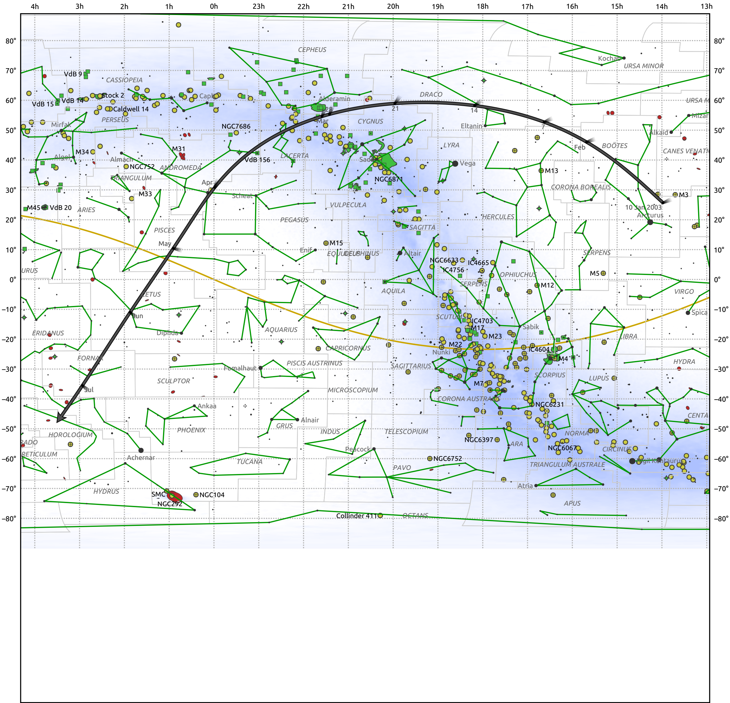
The path of C/2002 Y1 (Juels-Holvorcem) starting on 10 Jan 2003
