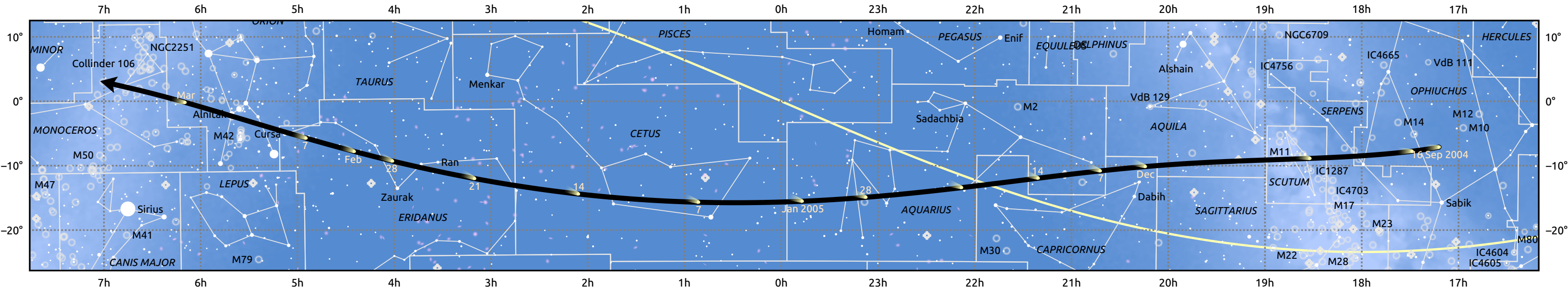
The path of 141P/Machholz starting on 16 Sep 2004
