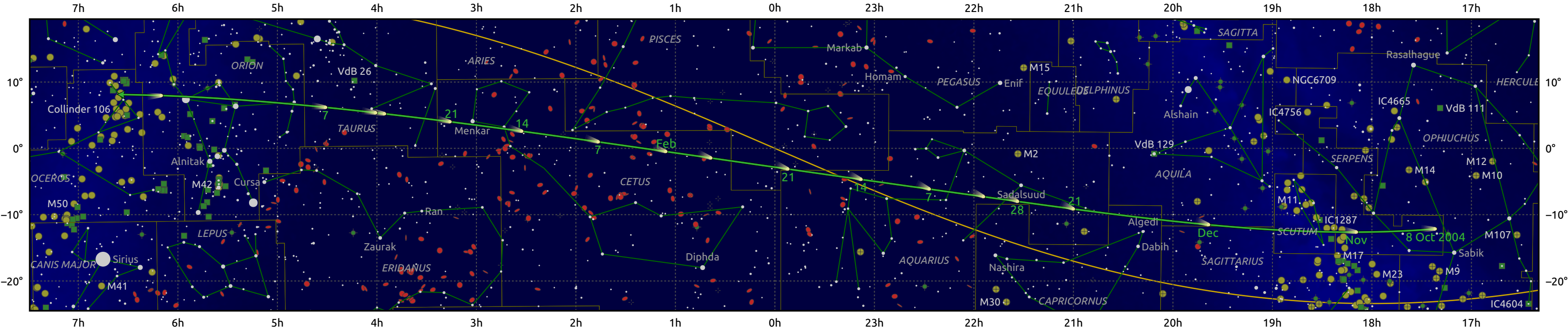
The path of 141P/Machholz starting on 8 Oct 2004
