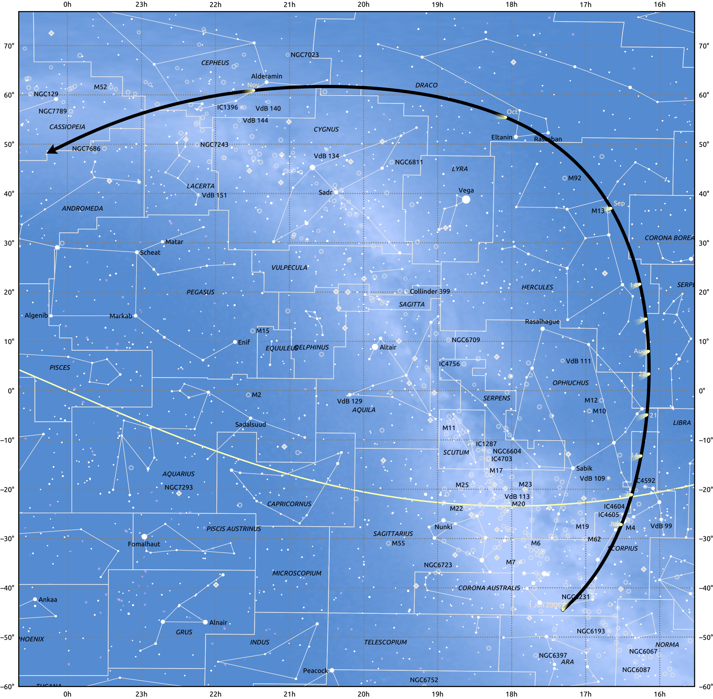
The path of 177P/Barnard starting on 31 May 2006
