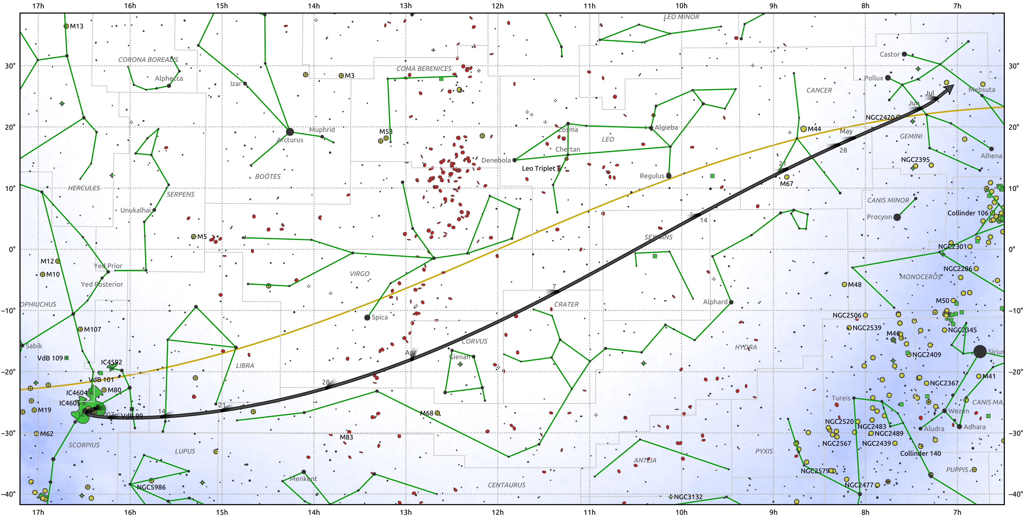
The path of C/2007 E1 (Garradd) starting on 10 Jan 2007
