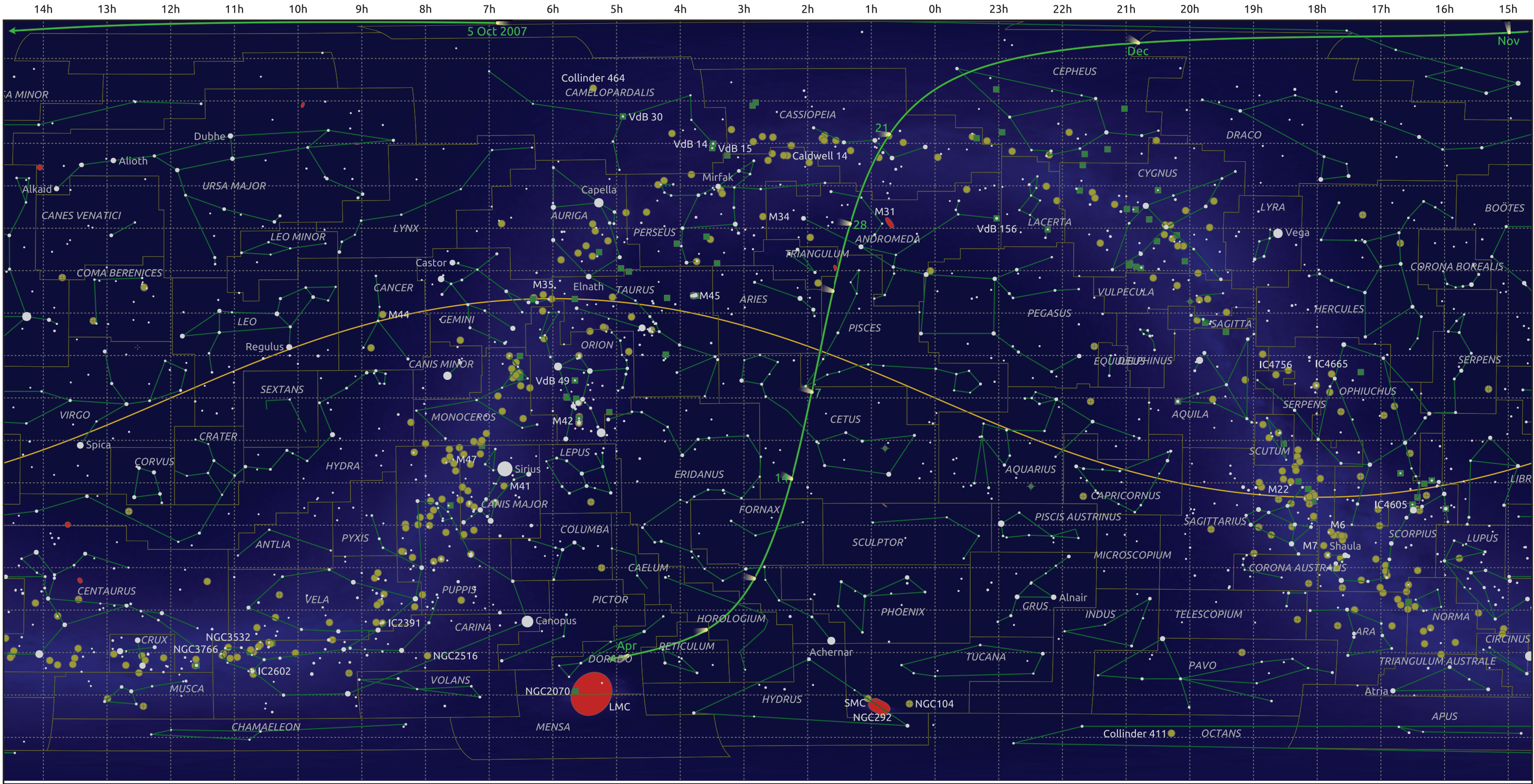
The path of 8P/Tuttle starting on 5 Oct 2007
