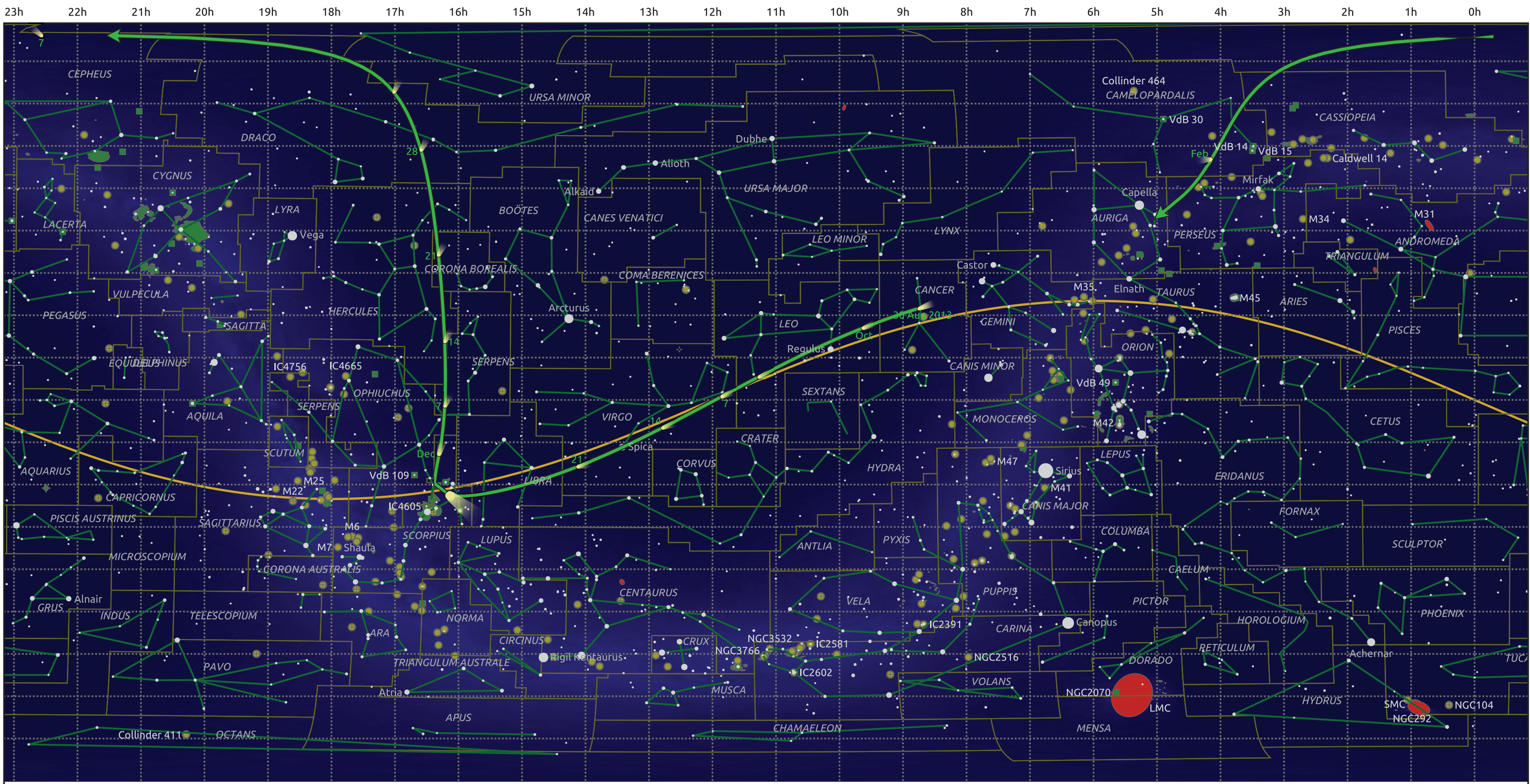
The path of C/2012 S1 (ISON) starting on 30 Aug 2013
