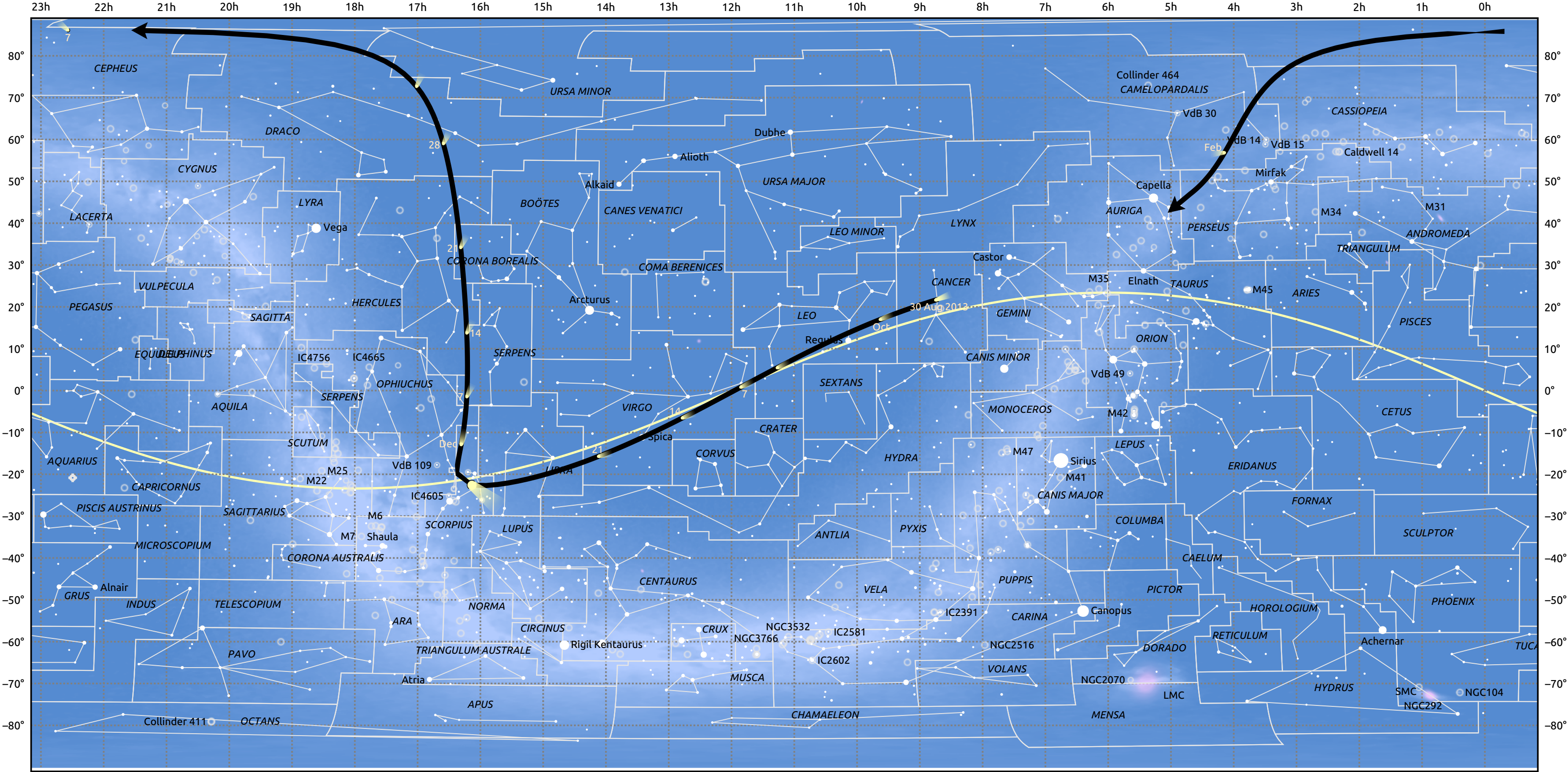
The path of C/2012 S1 (ISON) starting on 30 Aug 2013
