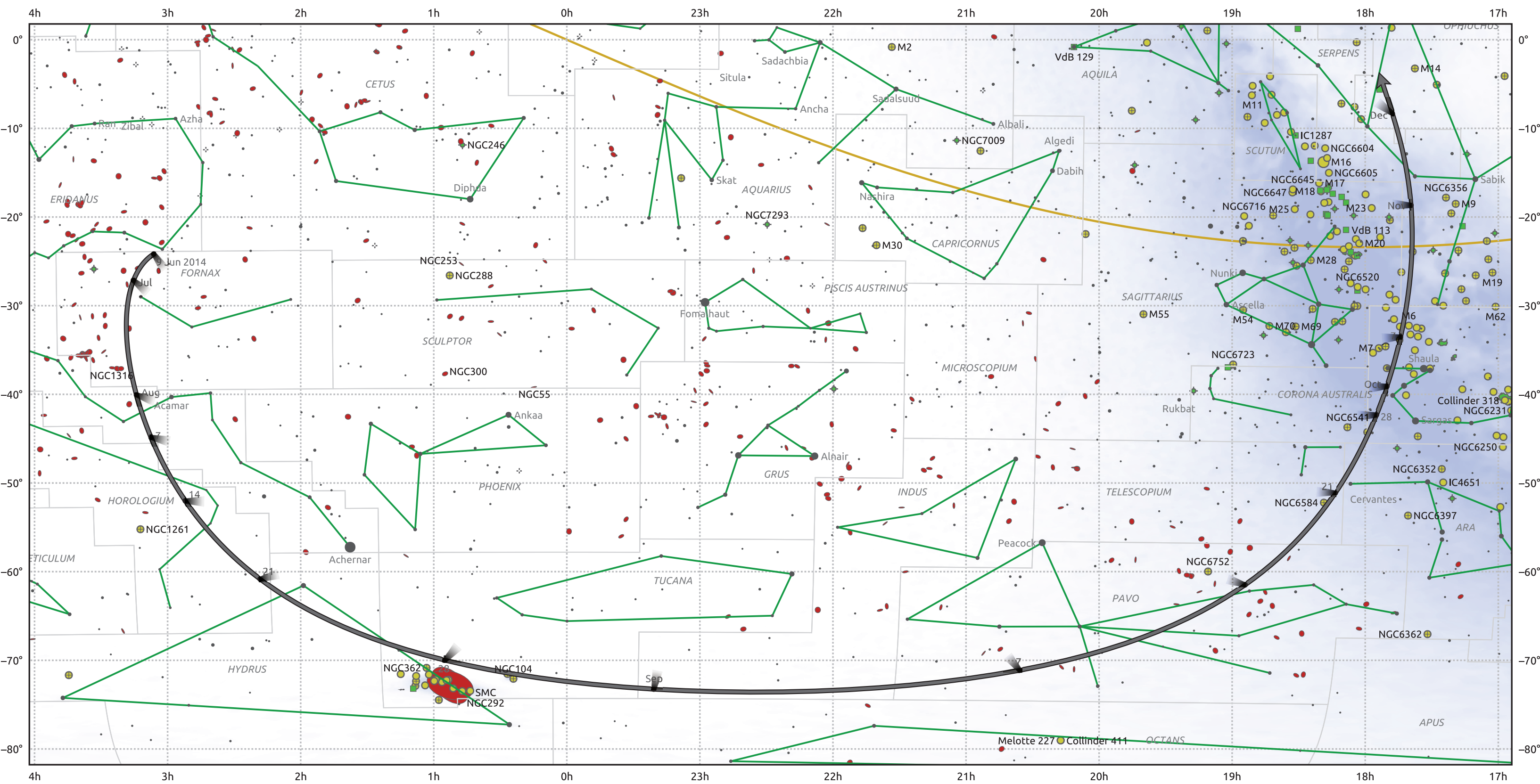
The path of C/2013 A1 (Siding Spring) starting on 9 Jun 2014
