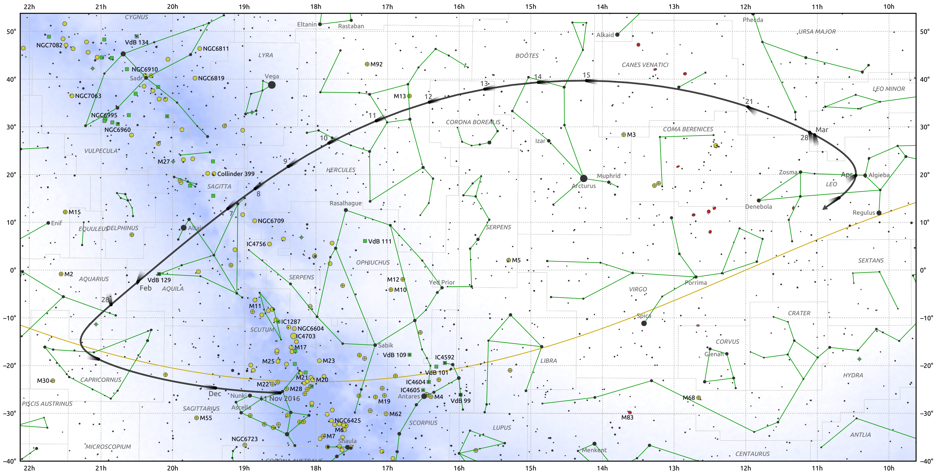
The path of 45P/Honda-Mrkos-Pajdusakova starting on 11 Nov 2016
