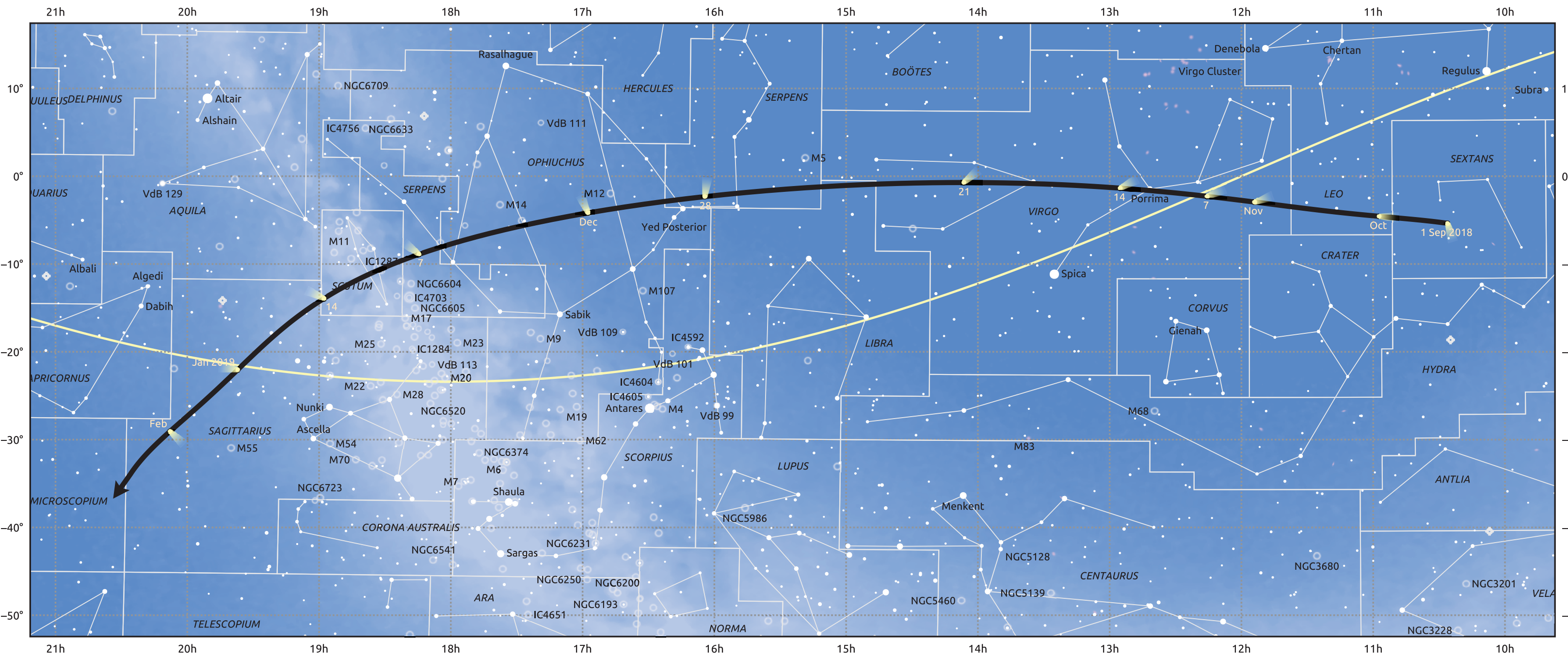
The path of C/2018 V1 (Machholz-Fujikawa-Iwamoto) starting on 1 Sep 2018
