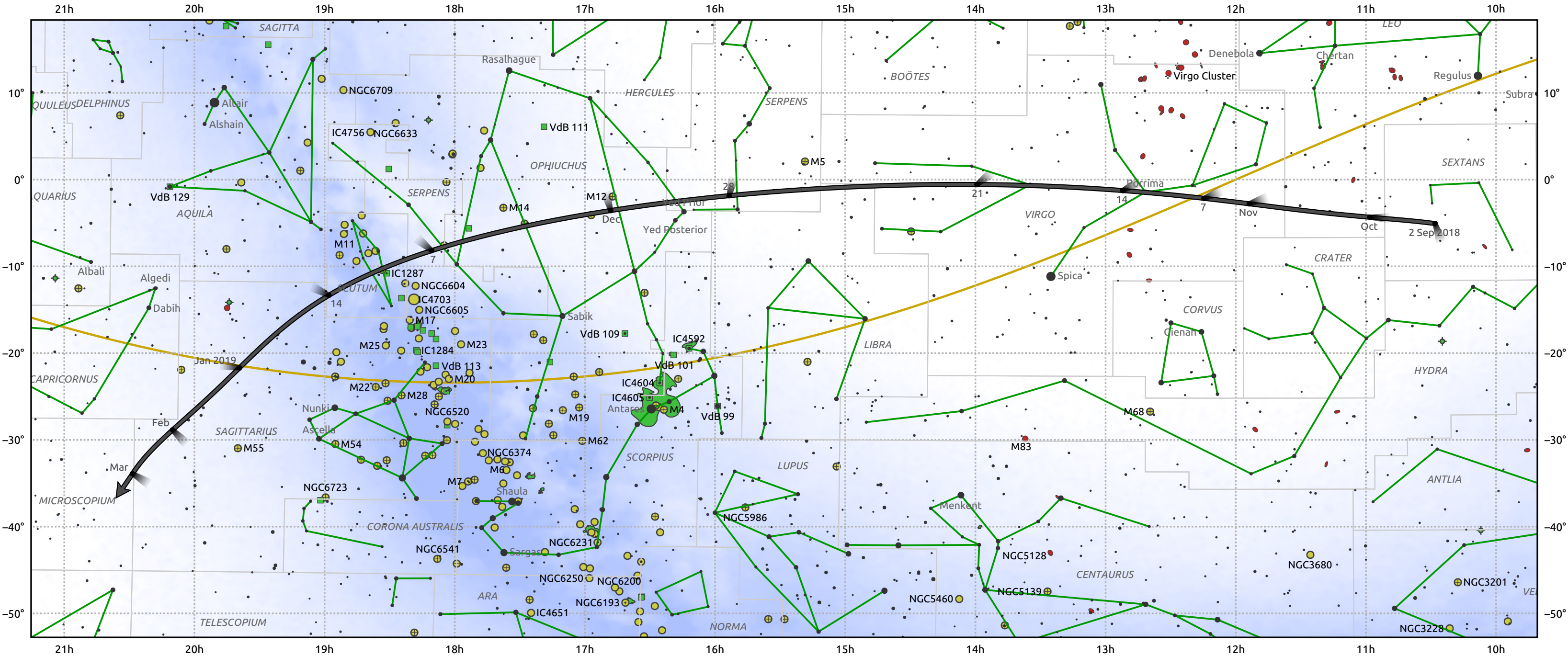
The path of C/2018 V1 (Machholz-Fujikawa-Iwamoto) starting on 2 Sep 2018
