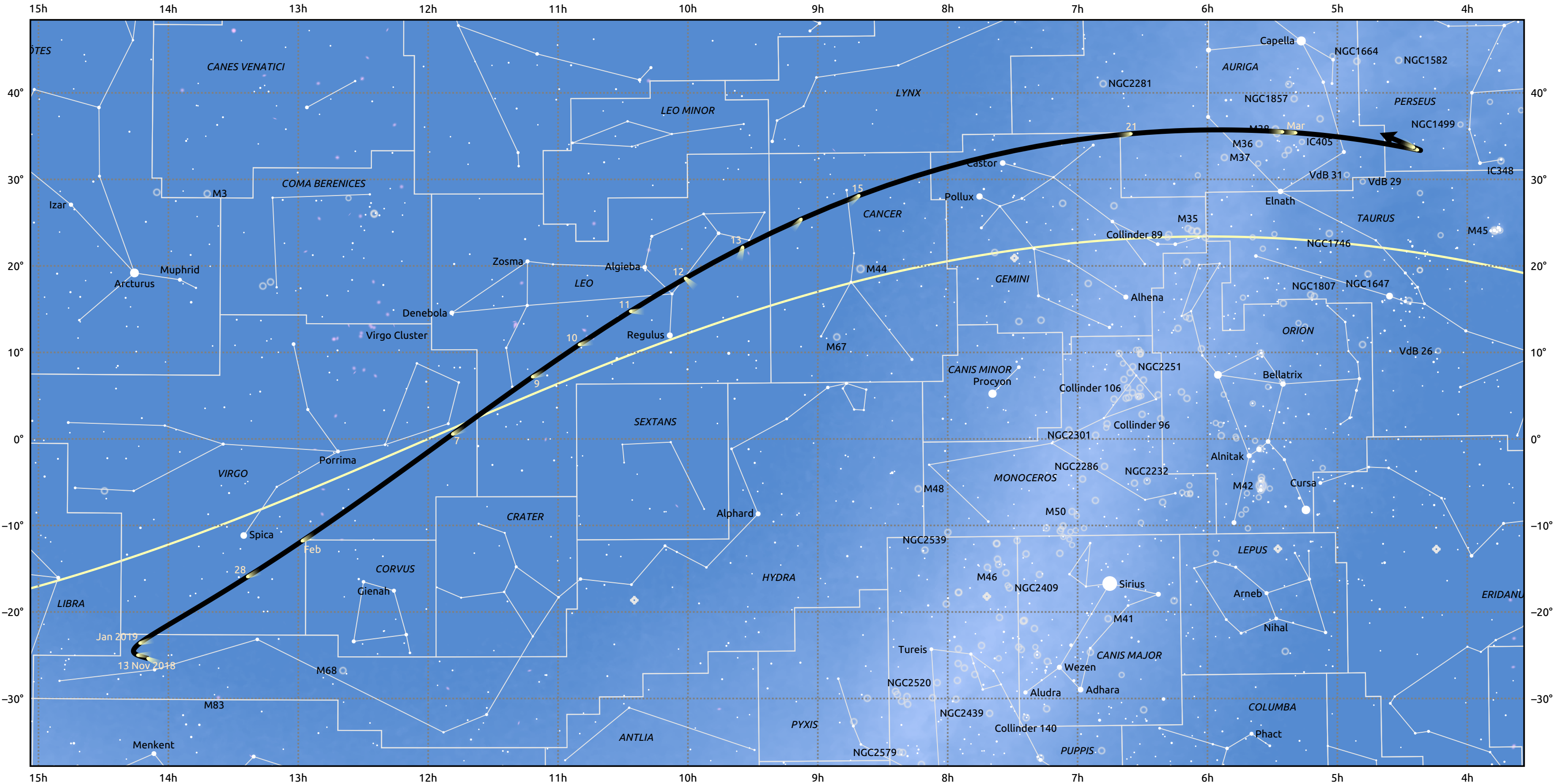
The path of C/2018 Y1 (Iwamoto) starting on 13 Nov 2018
