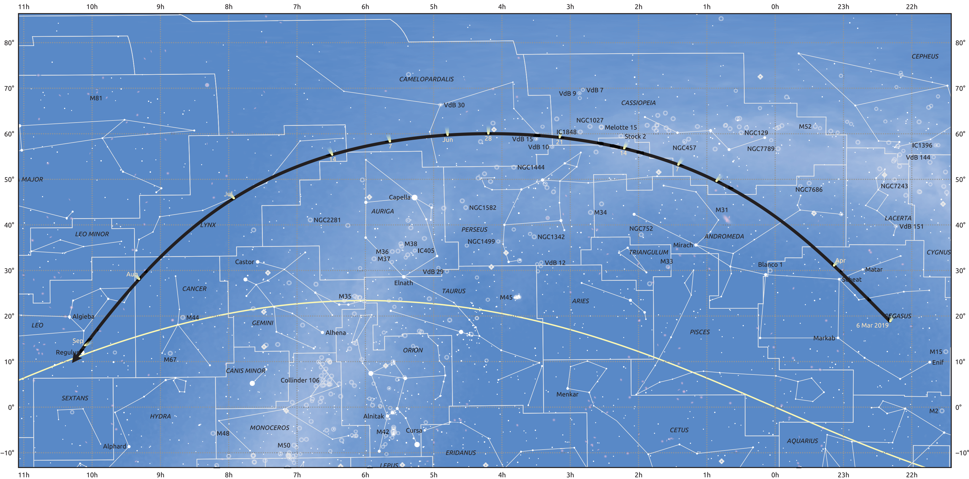
The path of C/2018 R3 (Lemmon) starting on 6 Mar 2019
