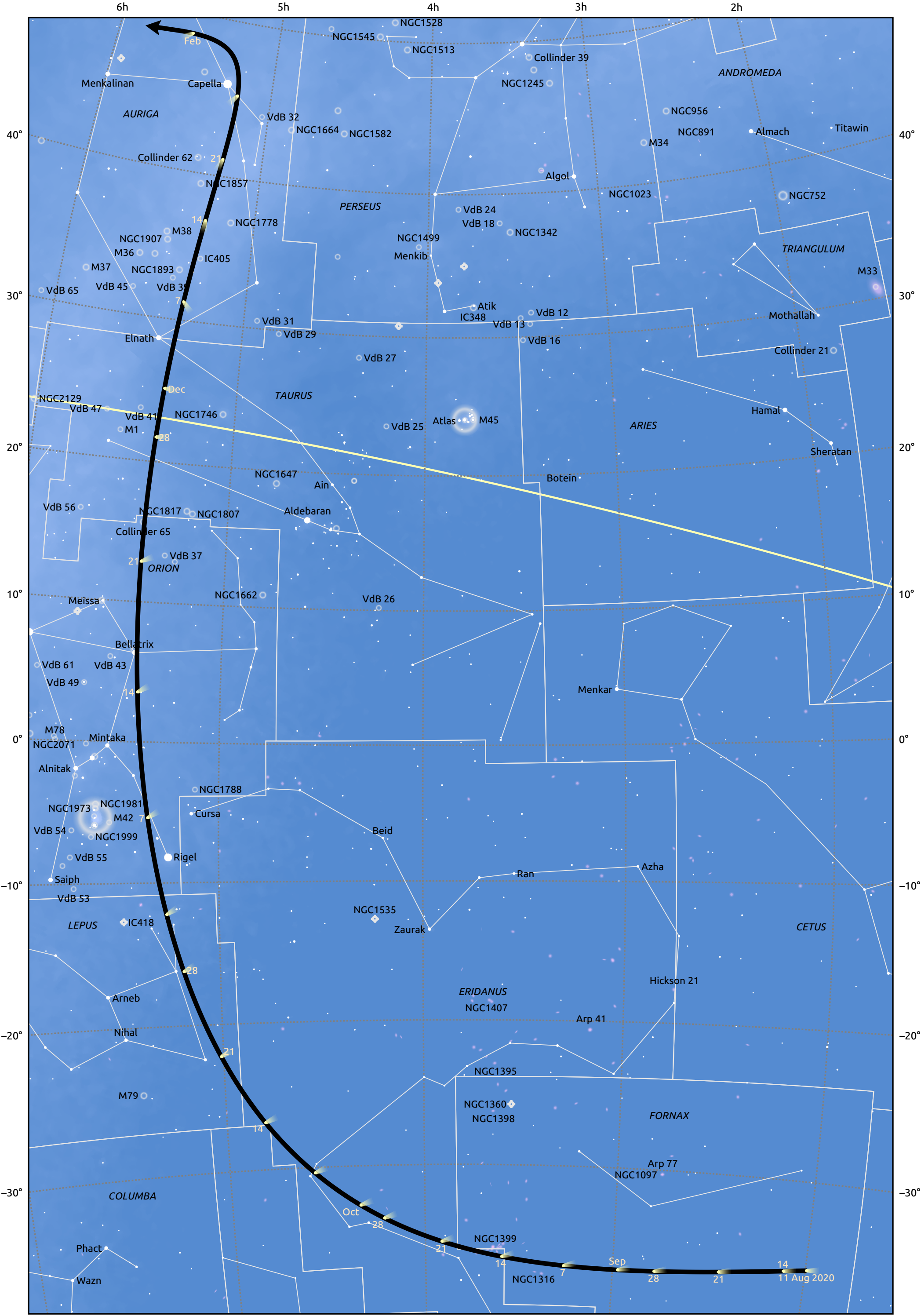
The path of C/2020 M3 (ATLAS) starting on 11 Aug 2020
