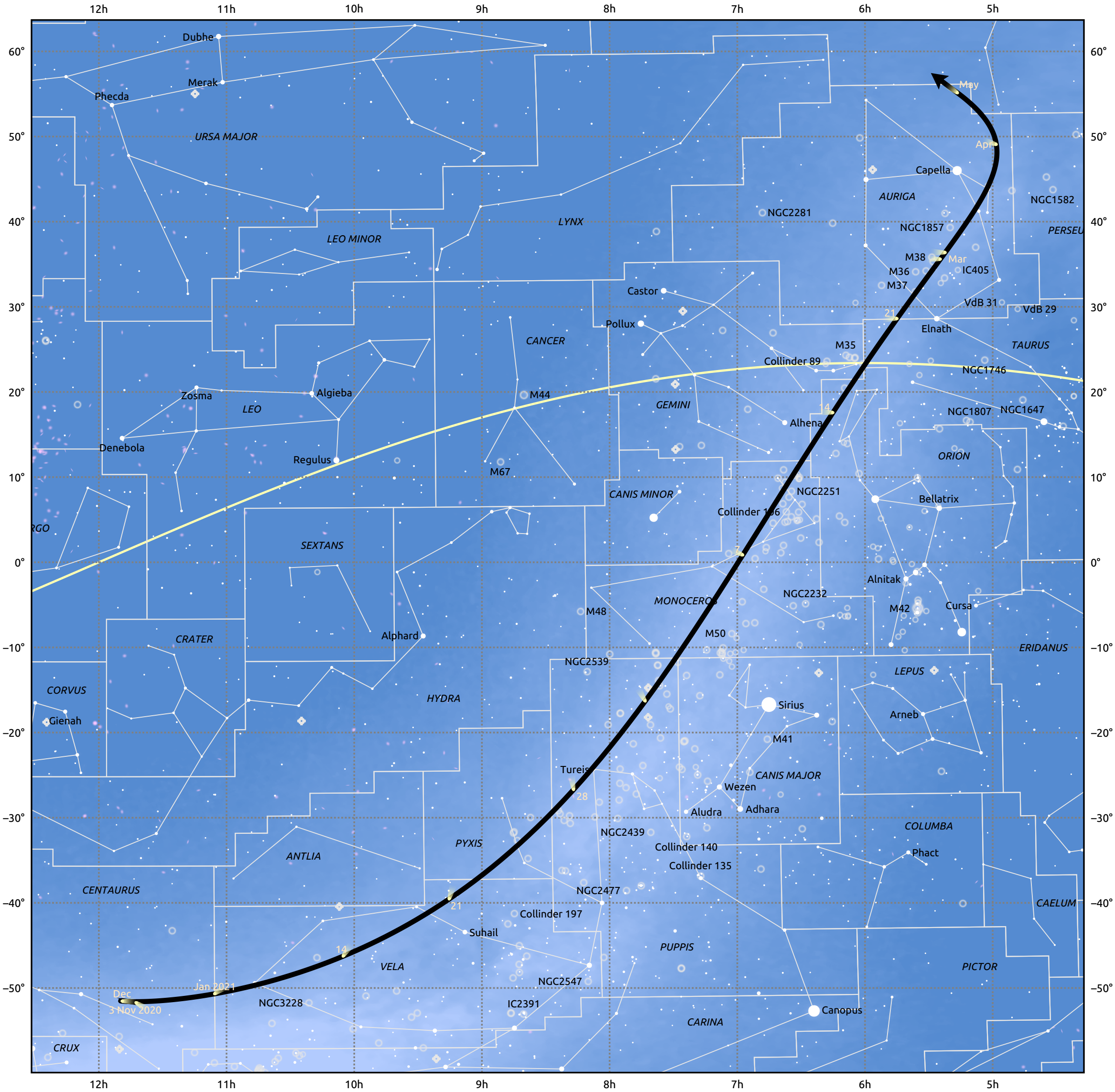
The path of C/2021 A2 (NEOWISE) starting on 3 Nov 2020
