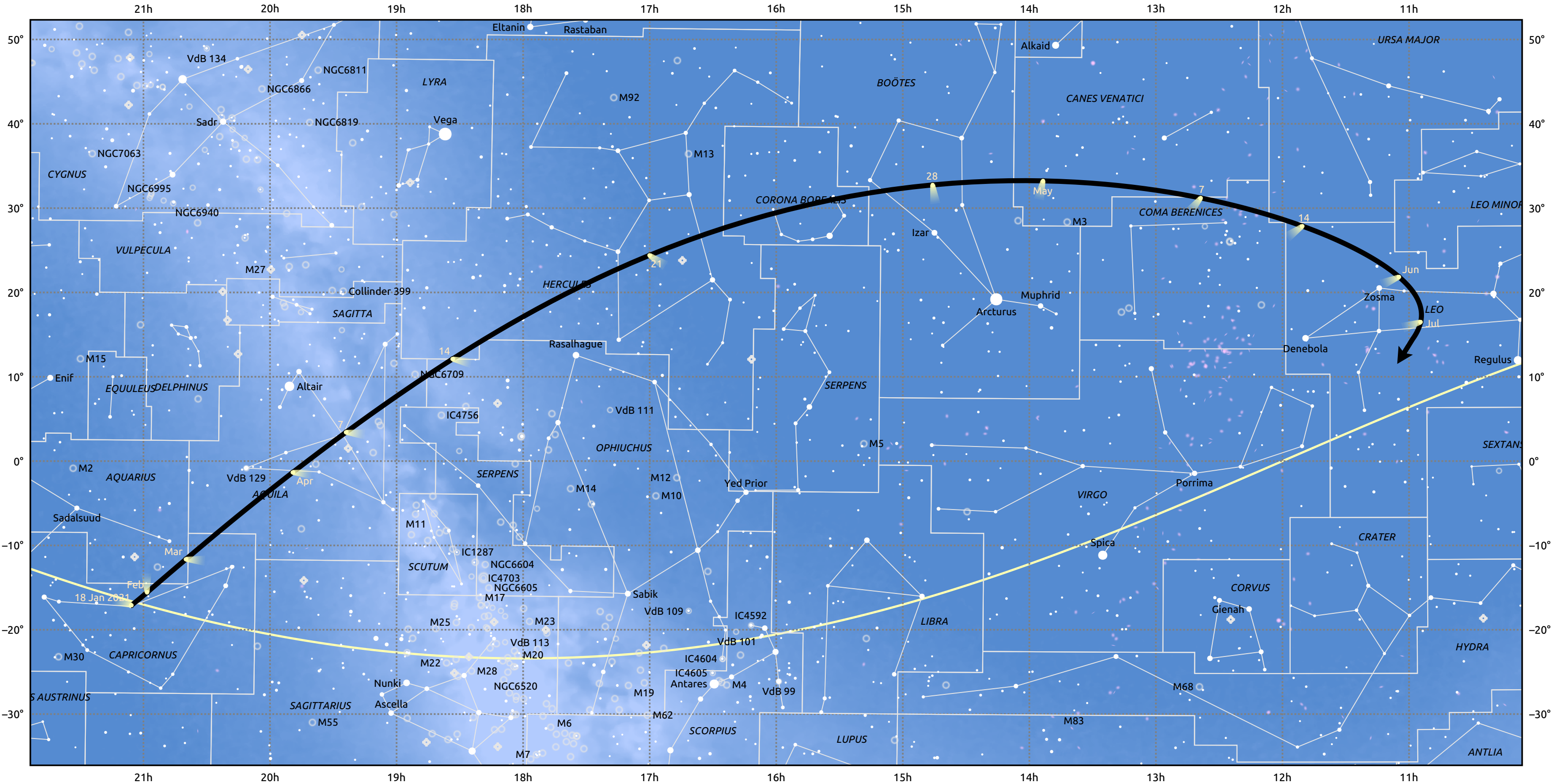
The path of C/2020 R4 (ATLAS) starting on 18 Jan 2021
