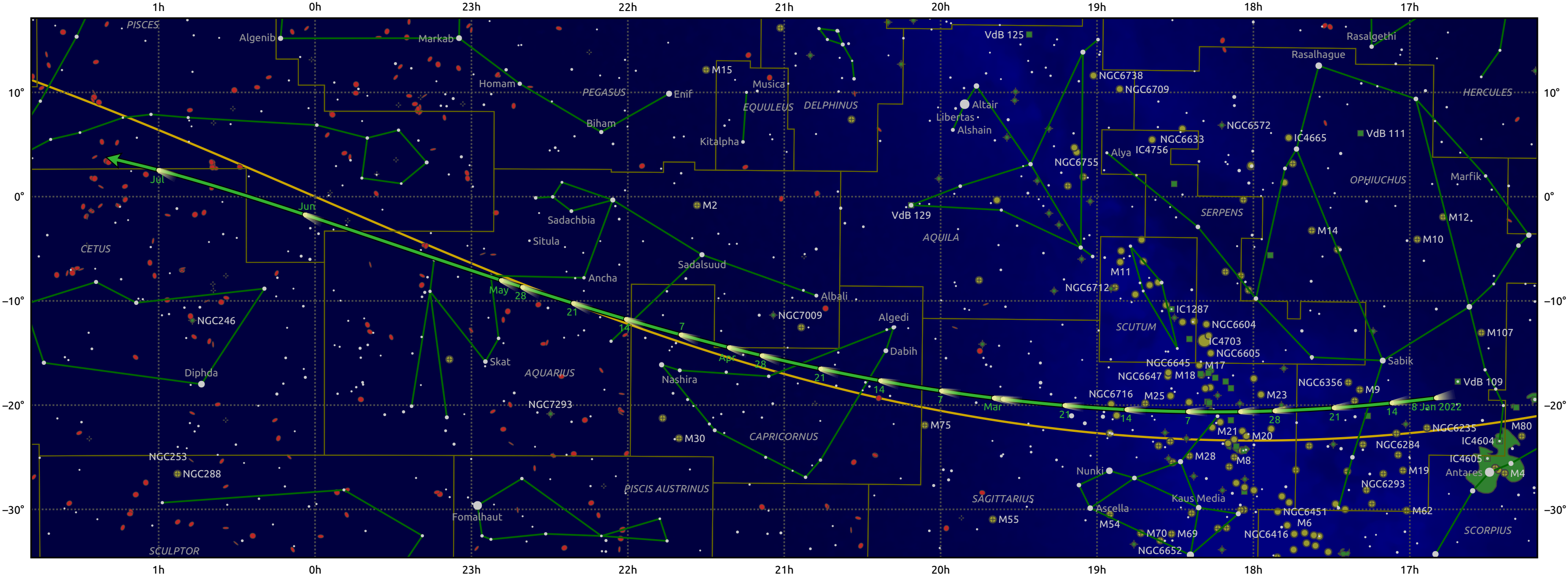
The path of 22P/Kopff starting on 8 Jan 2022
