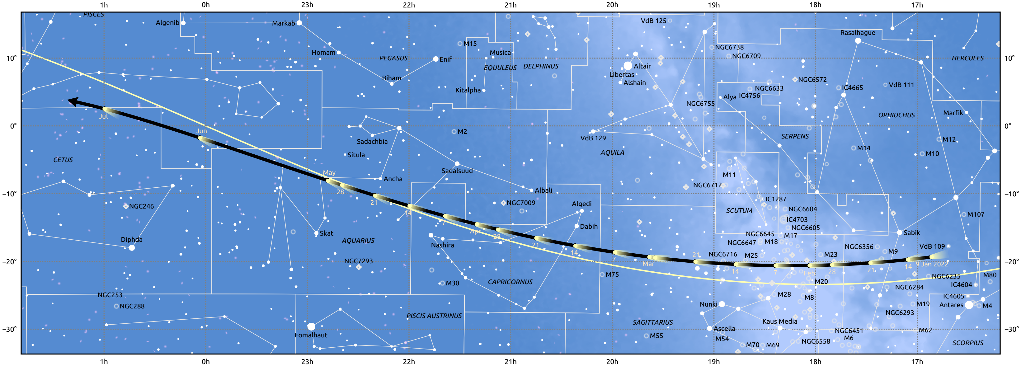
The path of 22P/Kopff starting on 9 Jan 2022
