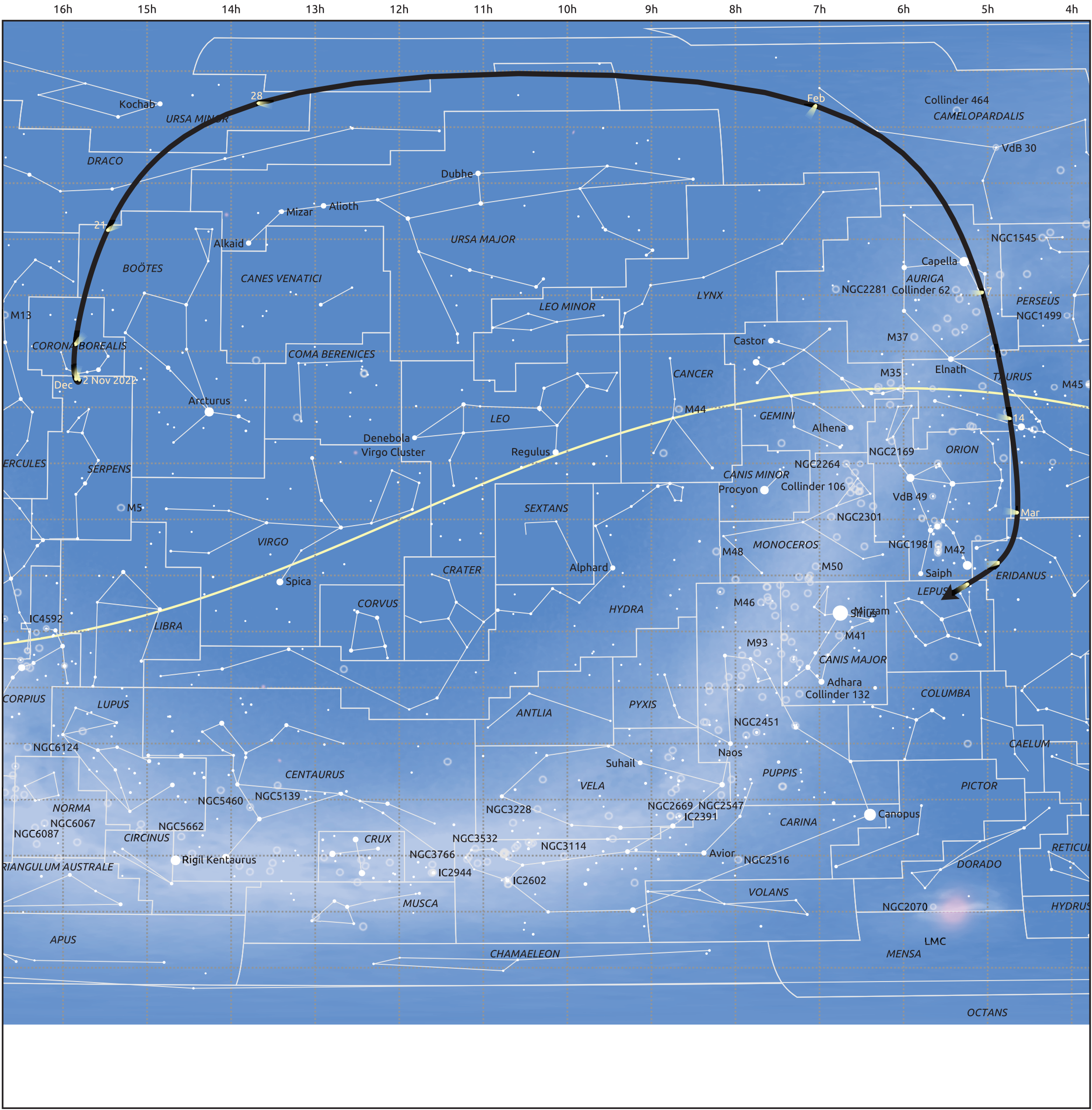
The path of C/2022 E3 (ZTF) starting on 2 Nov 2022
