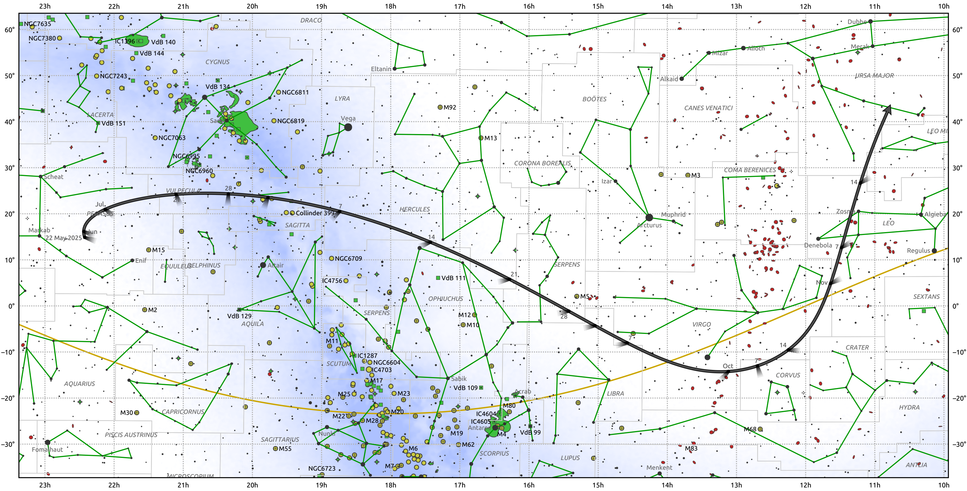
The path of C/2025 K1 (ATLAS) starting on 22 May 2025
