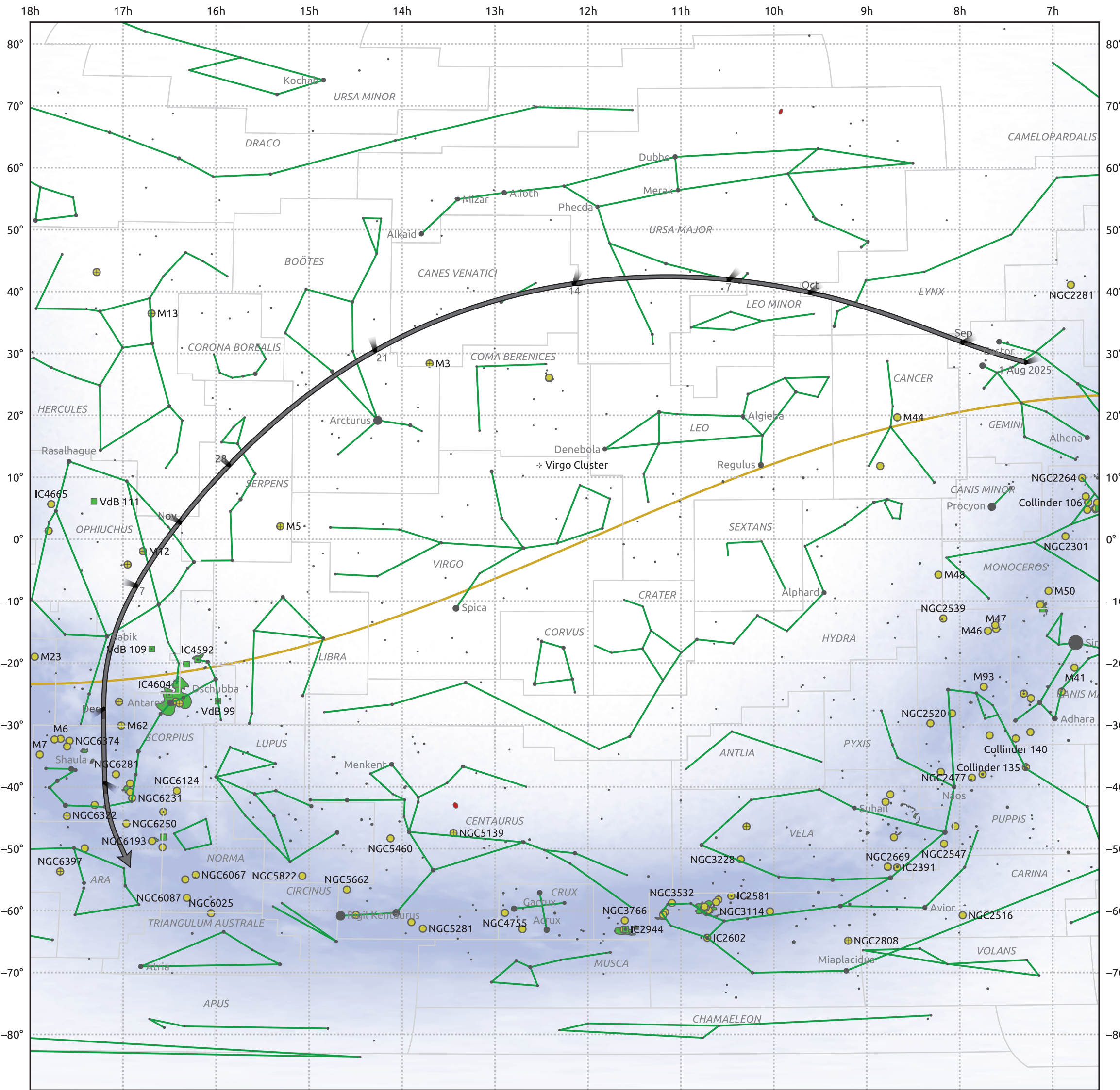
The path of C/2025 A6 (Lemmon) starting on 1 Aug 2025
