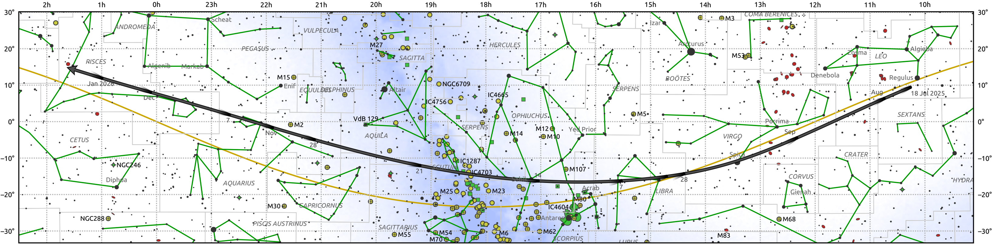
The path of C/2025 R2 (SWAN) starting on 18 Jul 2025
