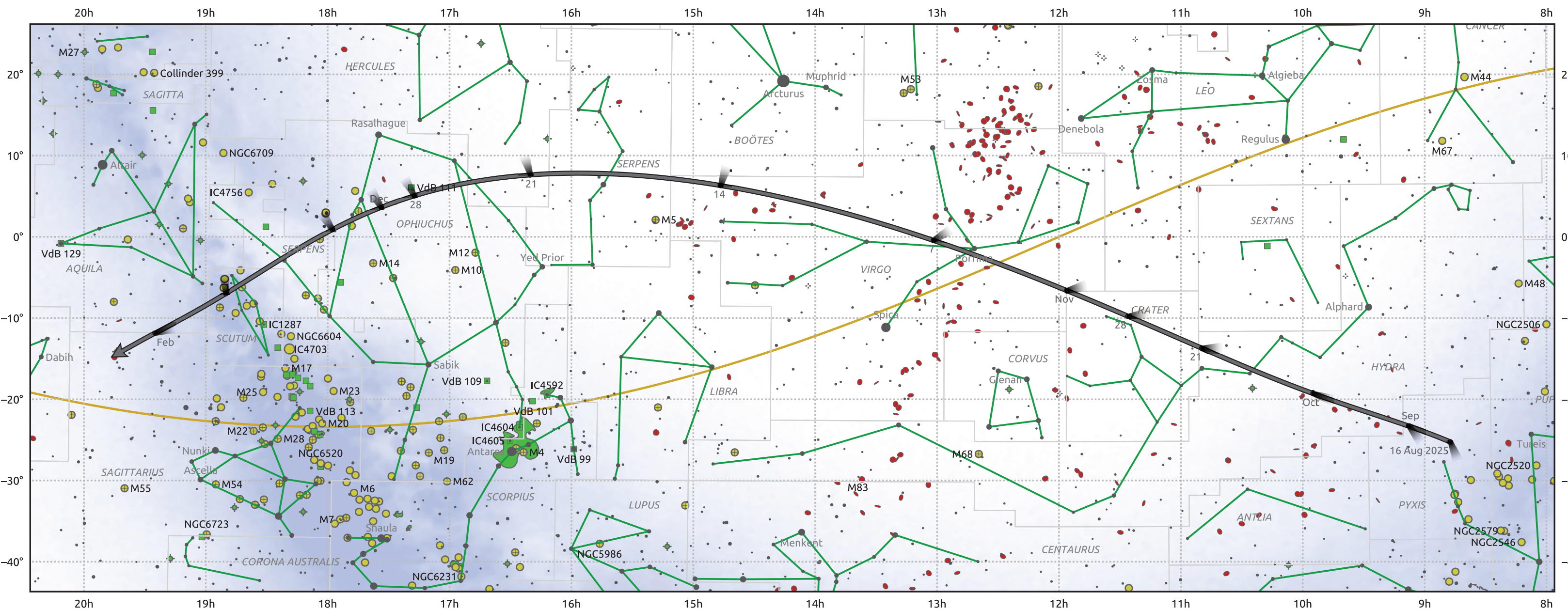
The path of C/2025 V1 (Borisov) starting on 16 Aug 2025
