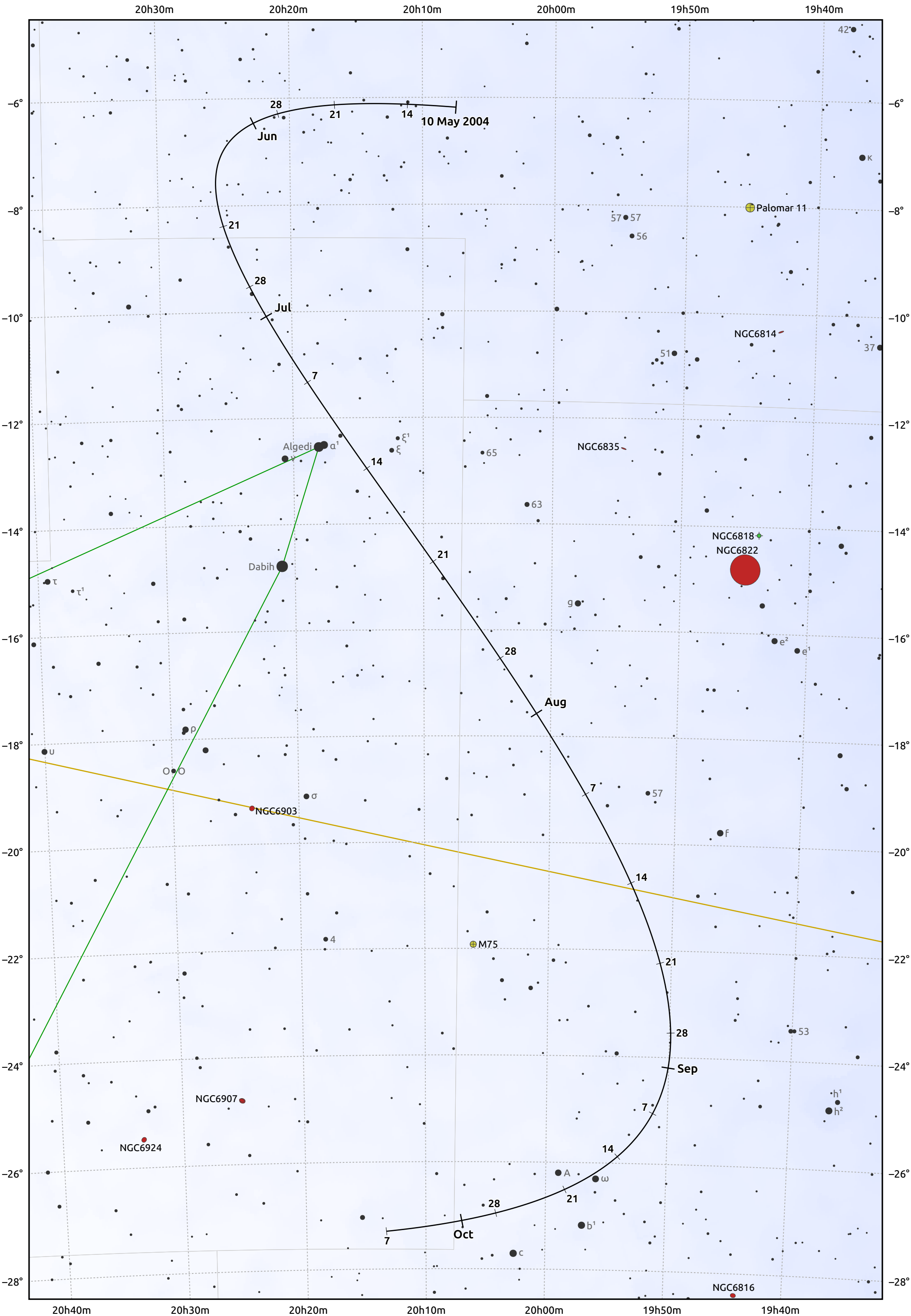
The path of Asteroid 387 Aquitania around opposition on 24 Jul 2004
