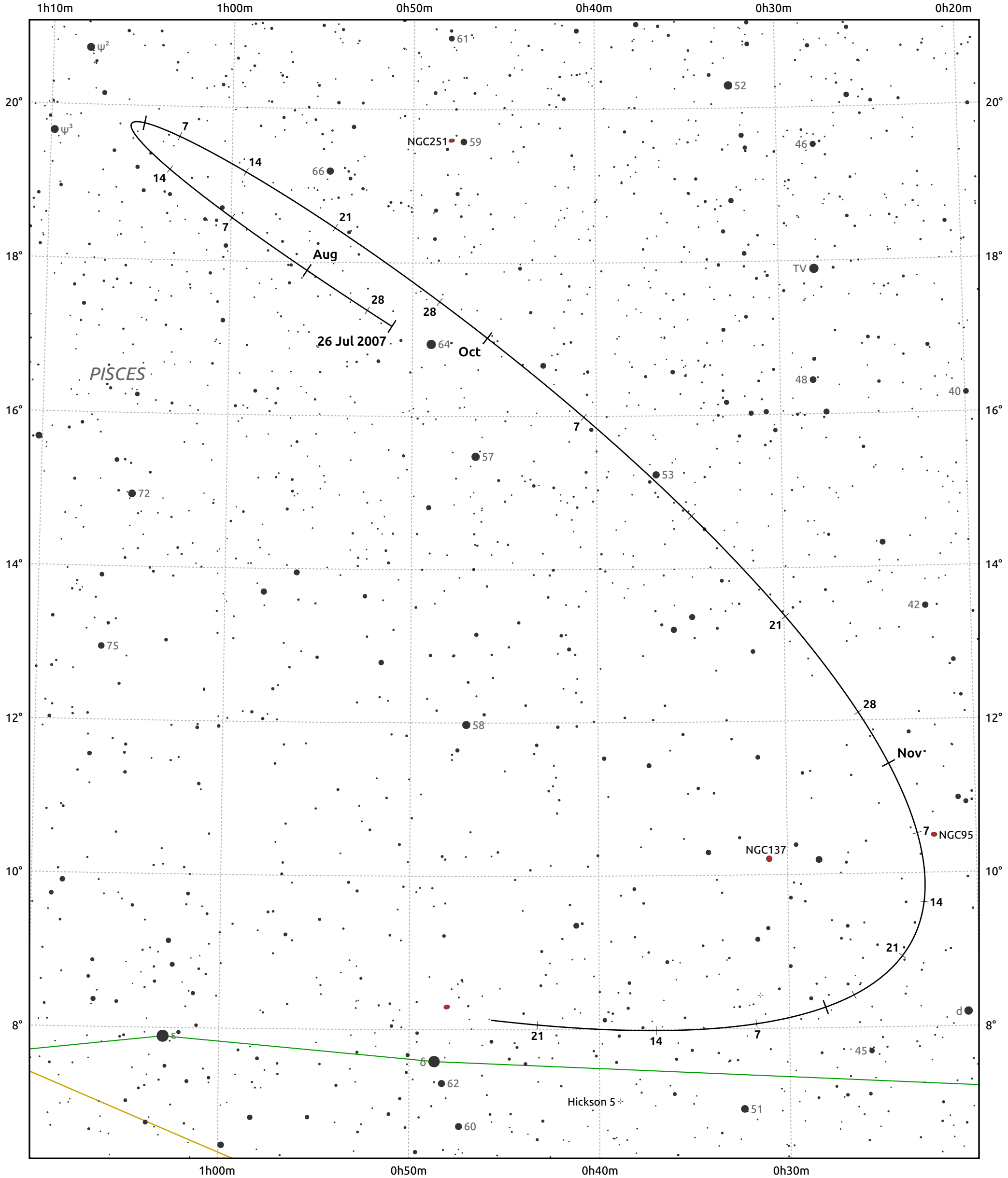
The path of Asteroid 12 Victoria around opposition on 9 Oct 2007
