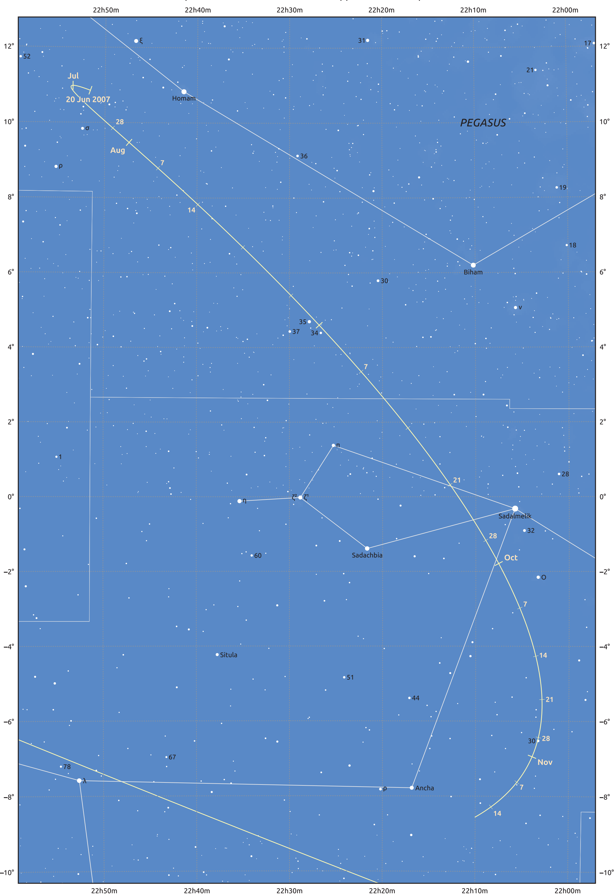
The path of Asteroid 2 Pallas around opposition on 3 Sep 2007
